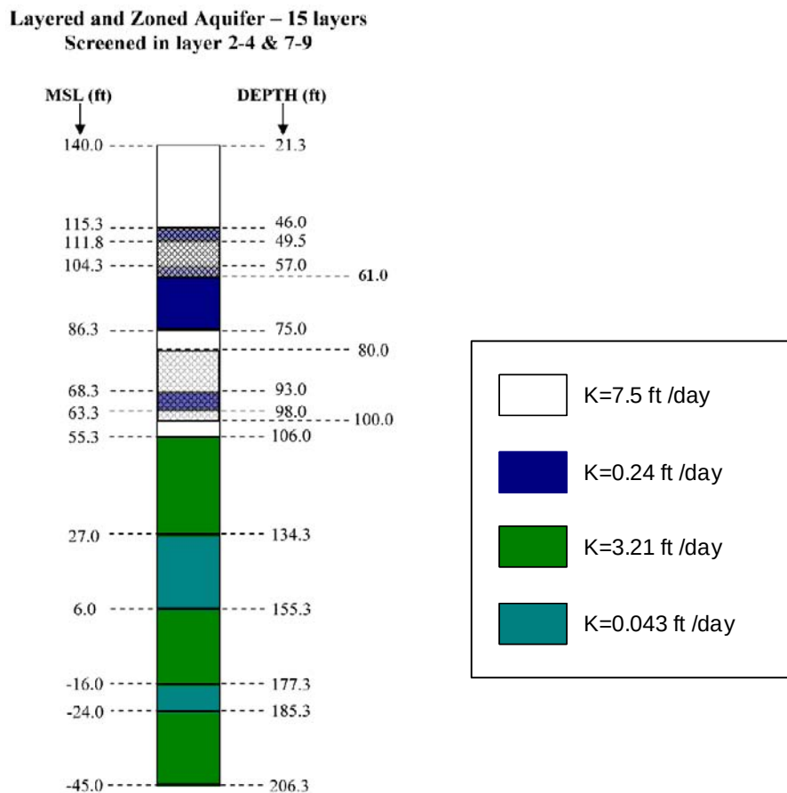
Figure 8. Conceptual model of demonstration site aquifer based on rotonsonic logs and pump tests.
