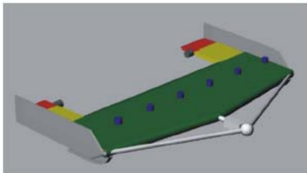
Figure 6. Perspective drawing of the 4-m sensor platform concept.
