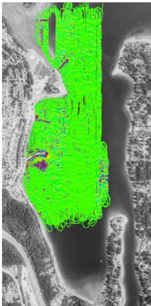
Figure 10. The MTA magnetometer survey superimposed on a recent aerial photograph of Ostrich Bay.
