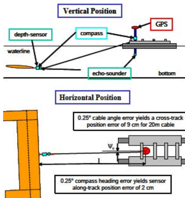
Figure 7. Sensor platform deployment concept resulting from SERDP Project UX-1322.
