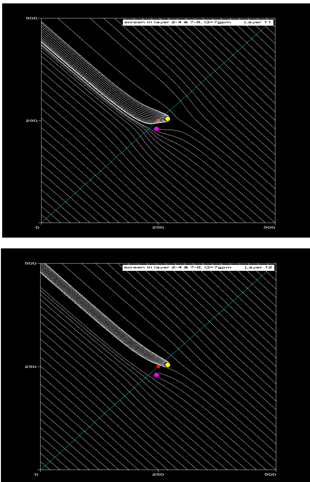
Figure E-28. Streamline Plan View in Layers 11&12. Scale is in ft and the layer designation is provided at the top right hand corner of each simulation.
