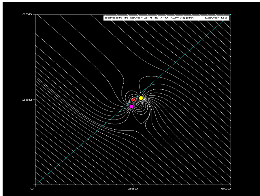
Figure E-24. Streamline Plan View in Layers 3&4. Scale is in ft and the layer designation is provided at the top right hand corner of each simulation.
