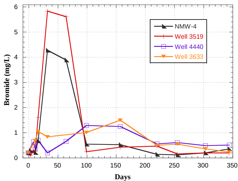
Figure 4.8. Tracer Test 2, HFTW-D: Bromide Concentrations in Deep Monitoring Wells Closest to the HFTWs – Row 1.
