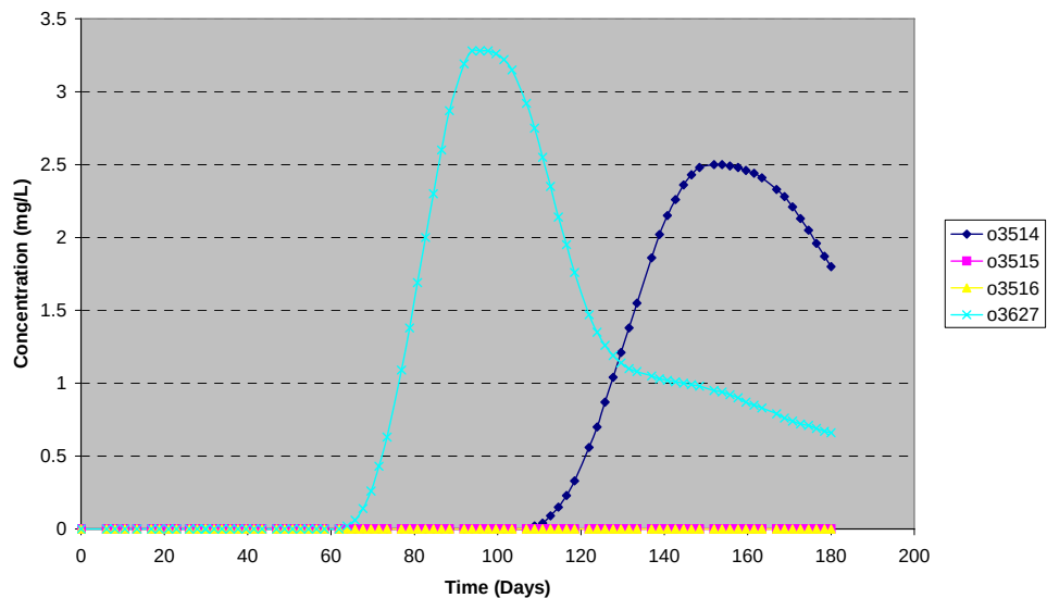
Figure E-10. Model Simulation of Bromide Concentrations in Far Downgradient Monitoring Wells 3514 and 3627. Wells 3515 and 3516 were not sampled due to screen depth.
