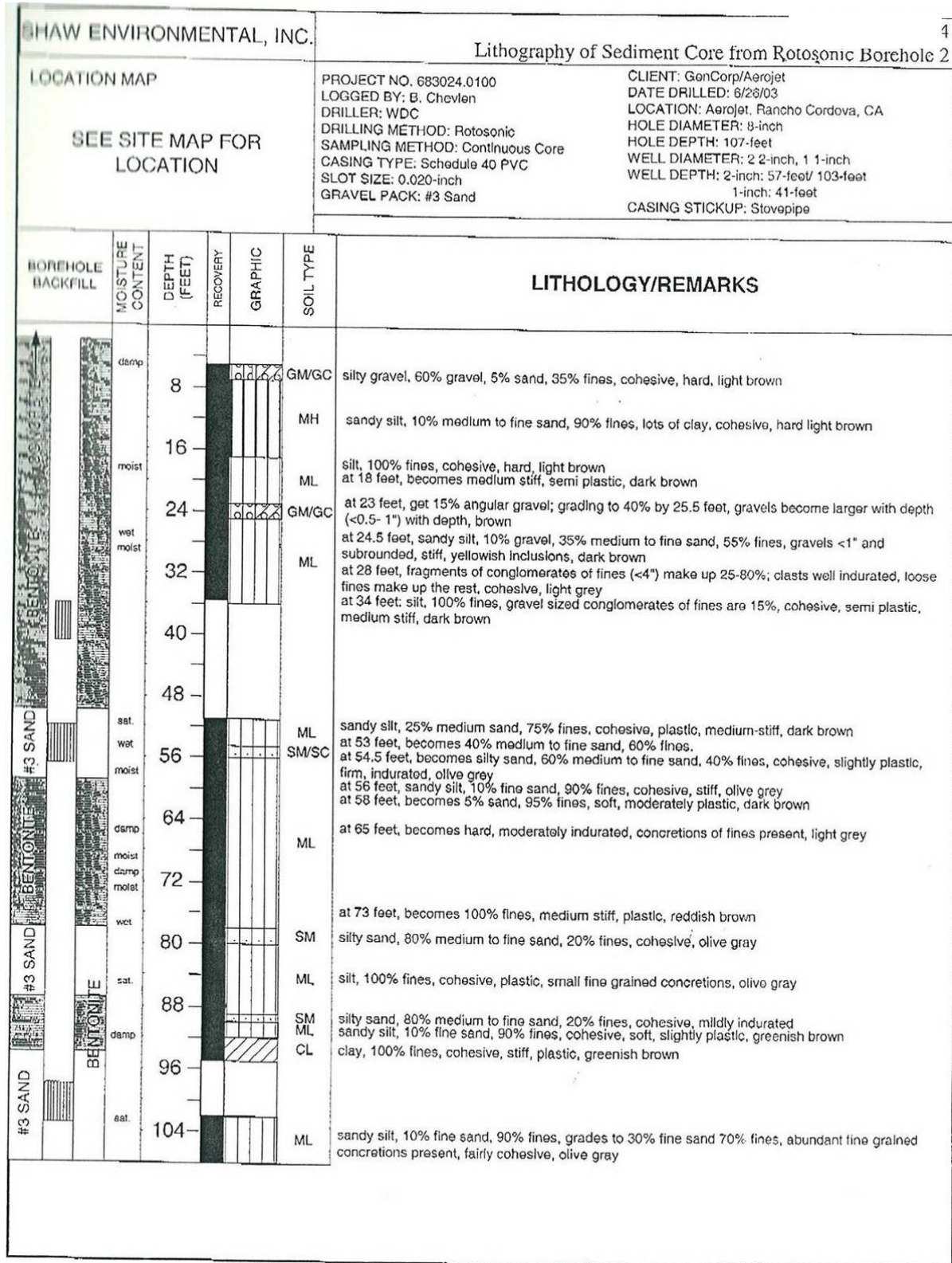
Figure 3.19. Lithography of Sediment Core from Borehole #2.
