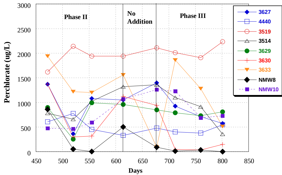
Figure 4.25. Perchlorate Levels in Deep Downgradient Monitoring Wells – Phase II & III.
