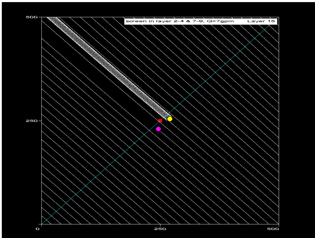
Figure E-30. Streamline Plan View in Layer 15. Scale is in ft and the layer designation is provided at the top right hand corner of each simulation.
