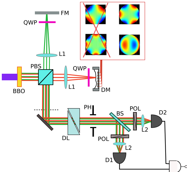
FIG. 1 (color online). Schematic of the experimental setup. Examples of aberrations induced by the deformable mirror are illustrated in the inset: the even-parity aberrations on the left are canceled, while the odd-parity ones on the right alter the shape of the interference pattern.
