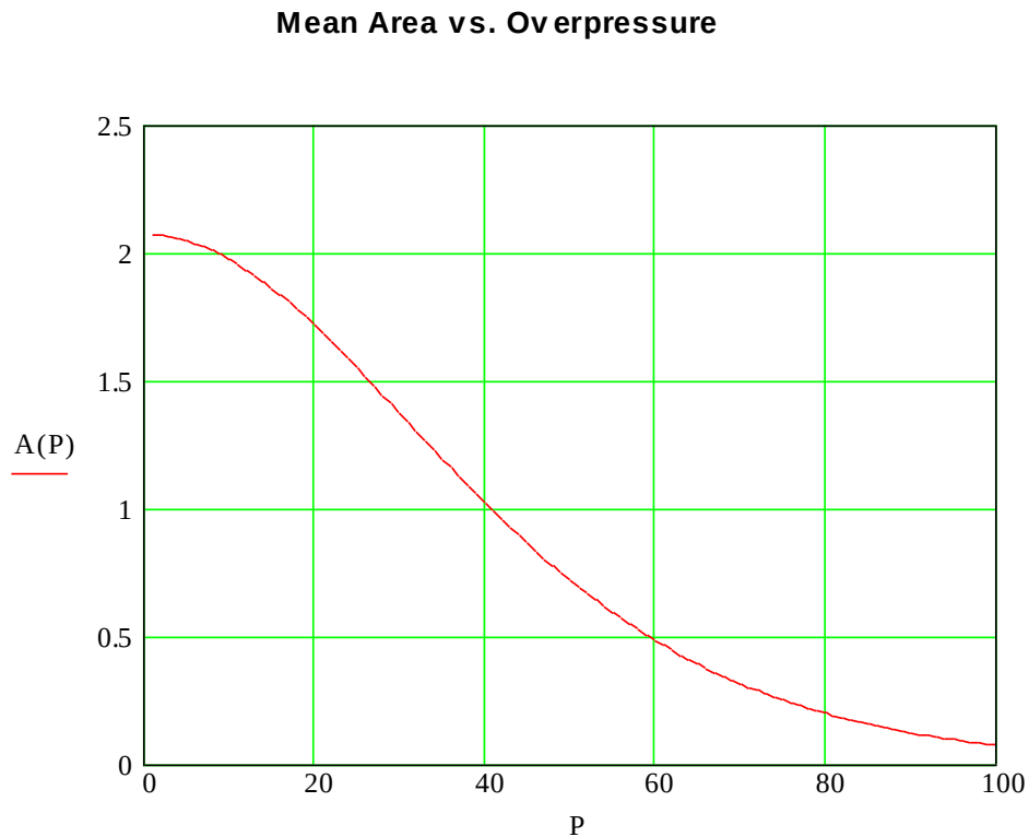
FIGURE 3-29. Distribution of Average Glass Fragments Area vs. Blast Overpressures
