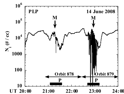
Figure 2. PLP plasma densities measured between 20:00 and 24:00 UT on 14 June 2008. Times of C/NOFS orbits 878 and 879 are indicated along with midnight (M) and perigee (P) crossings. Solid bars mark intervals when C/NOFS was in darkness.
