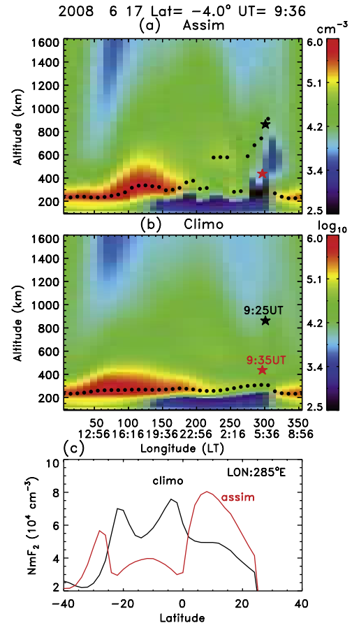
Figure 3. (a) 2D density map obtained from the assimilation model, where the x- and y- axis represent longitude and altitude, respectively. (b) 2D density map based on the climatology model output. The black and red star symbols in Figures 3a and 3b denote the DMSP-F17 and C/NOFS satellite locations when the minimum densities were observed at 9:25 and 9:35 UT, respectively. The black dots indicate local h_m F_2 . (c) 1D plot of N_m F_2 as a function of geographical latitude, where the red and black lines represent results from the assimilation and climatology models, respectively.
