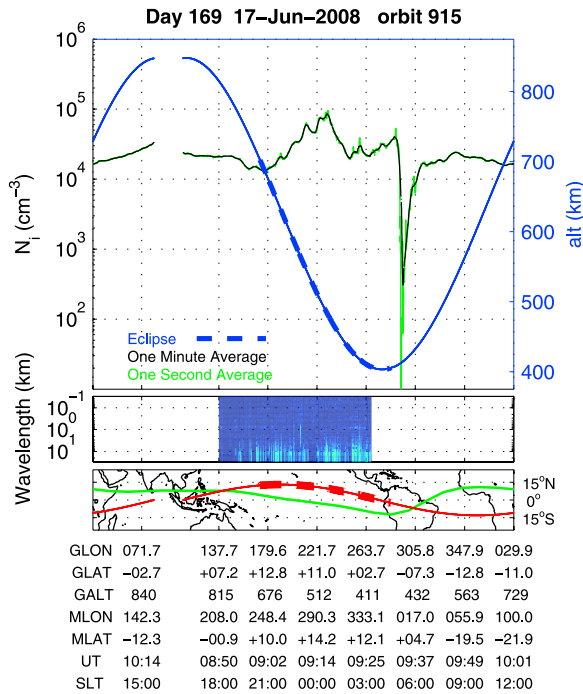
Figure 1. Dawn plasma depletion, orbit 915, Jun 17, 2008. (top) 1-min integrated ionospheric density (black), 1-s integrated density (green), satellite altitude (blue). Middle panel: FFT from the 512 Hz PLP data. (bottom) Map with satellite trajectory (red) and magnetic equator (green). Thicker dotted lines indicate when C/NOFS was in darkness.
