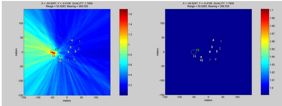
Figure 28. Acoustic localization of a single black-capped vireo song, using a 12-channel microphone array. Numbers in white indicate positions of microphones that were used in computing the location estimate; numbers in gray indicate microphones that were not used due to inadequate received signal level. The circle indicates the estimated location. Left: Colors indicate the sum of the cross-correlation functions from all pairs of microphones for each point in space. The highest value is the estimated location of the singing bird. Right: Same data, with colors scaled so that the red area (within the circle) indicates a 95% confidence interval around the estimated location.
