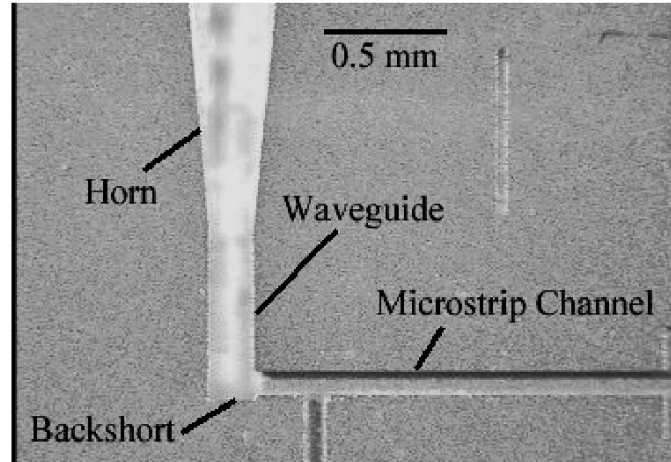
Figure 11. (a) W-band waveguide housing showing the microstrip probe circuit, STNO chip, and output waveguide. (b) Photograph showing the output horn antenna, microstrip channel, and waveguide section.
