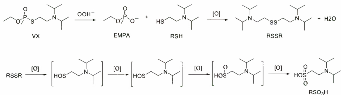
Scheme 2. RSO 3 H
