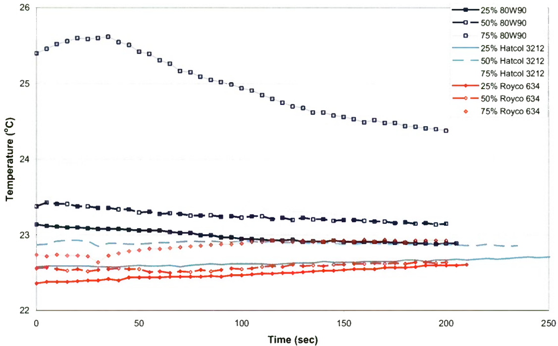
Figure 11. Observed Temperature Changes for DDC/Cold-Weather Kit Mixed with POLs
