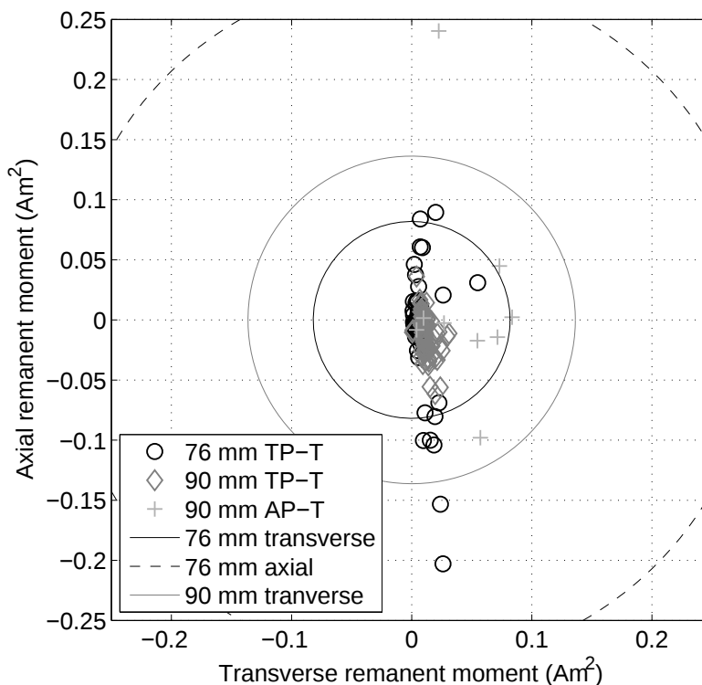
Figure 1. Remanent magnetization of 76 and two types of 90 mm projectiles measured with the MRIP platform at Limestone Hills, MT. Remanent magnetizations are split into the component along the axis of the project (axial) and across the axis (perpendicular). Contours delineating the values of the induced magnetizations of the 76 and 90 mm projectiles (as previously measured at the U.S. Army Corps of Engineers (USACE) Engineer Research and Development Center (ERDC) test stand) are also shown. The axial induced magnetization for the 90 mm projectile is larger than the range of values shown on the plot.
