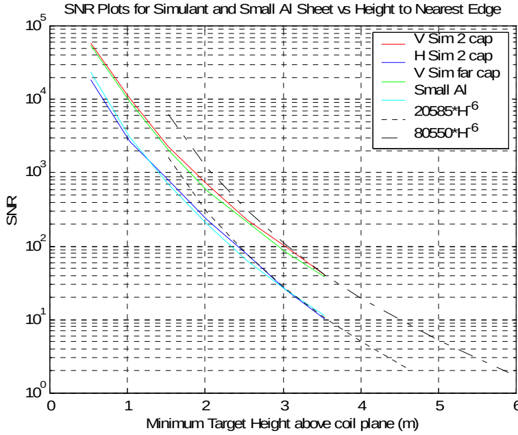
Figure 37. SNR plot for amplitude data shown in previous plot, displayed in linear-log format.
