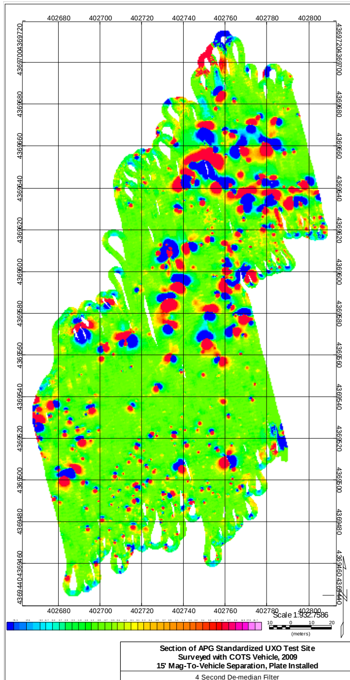
Figure 23: Legacy Area Surveyed with COTS Vehicle, Mags 15' Back, Skidplate Installed, with 4 Second De-median Filter Correction
