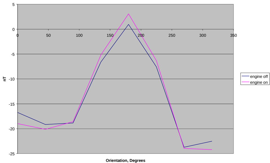
Figure 6: Octant Test, Mag 15' Behind vehicle, Skidplate Installed
