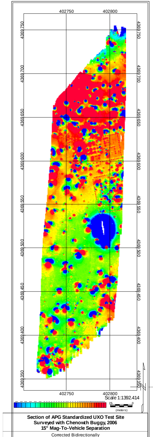
Figure 11: APG Site Legacy Area Section Surveyed in 2006 with Chenoweth Buggy, Mags 15' Back, with Bidirectional Correction
