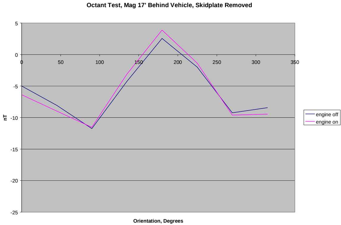
Figure 7: Octant Test, Mag 17' Behind Vehicle, Skidplate Removed
