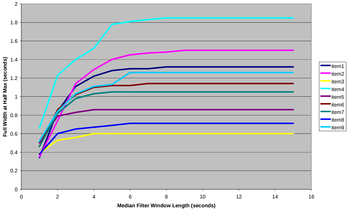
Figure 36: Nine Objects, Anomaly Full Width at Half Max as a Function of Median Filter Window Length
