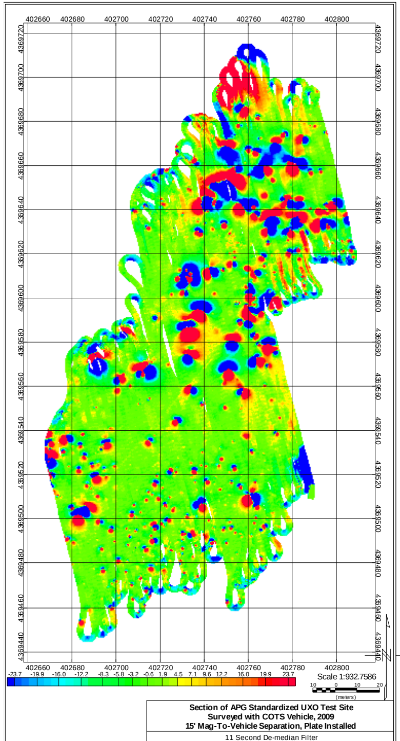
Figure 30: Legacy Area Surveyed with COTS Vehicle, Mags 15' Back, Skidplate Installed, with 11 Second De-median Filter Correction
