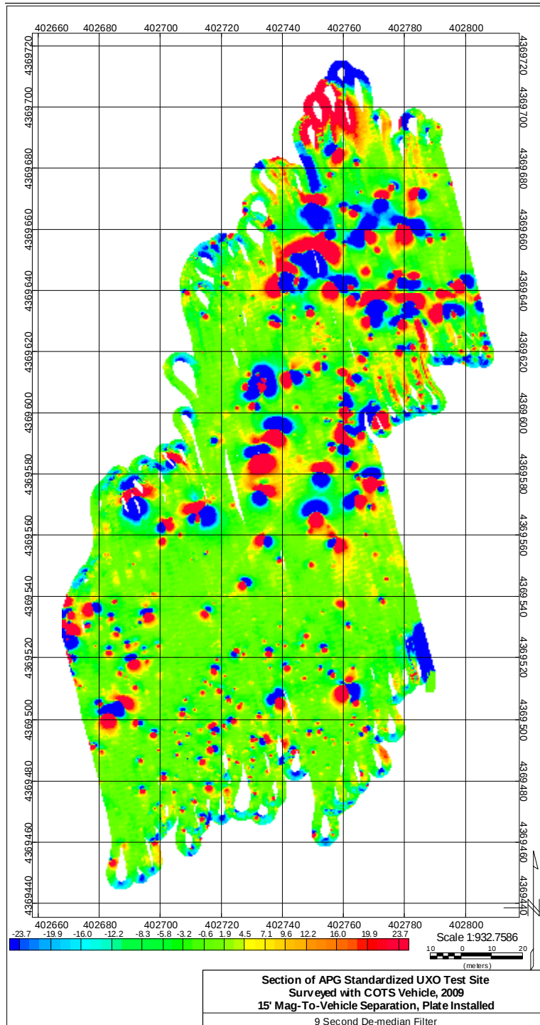
Figure 28: Legacy Area Surveyed with COTS Vehicle, Mags 15' Back, Skidplate Installed, with 9 Second De-median Filter Correction
