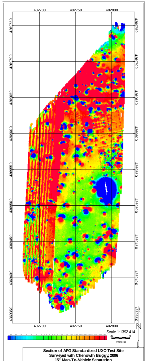
Figure 12: APG Site Legacy Area Plus Adjacent Section Surveyed in 2006 with Chenoweth Buggy, Mags 15' Back, with Bidirectional Correction
