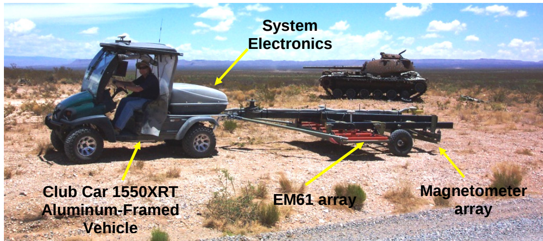
Figure 4: Club Car 1550XRT towing the VSEMS platform
