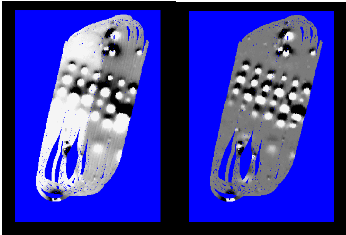
Figure 2: Sample unfiltered (left) and filtered (right) data taken with one of several UTVs tested (a Yamaha Rhino, mags 20' back) at the Devens Test Site, clearly showing the heading-dependent effect of vehicle signature. The image on the left has approximately 40nT of bulk signature. The image on the right has had bulk signature removed through de-median filtering. Image scale is \pm 50 nT.
