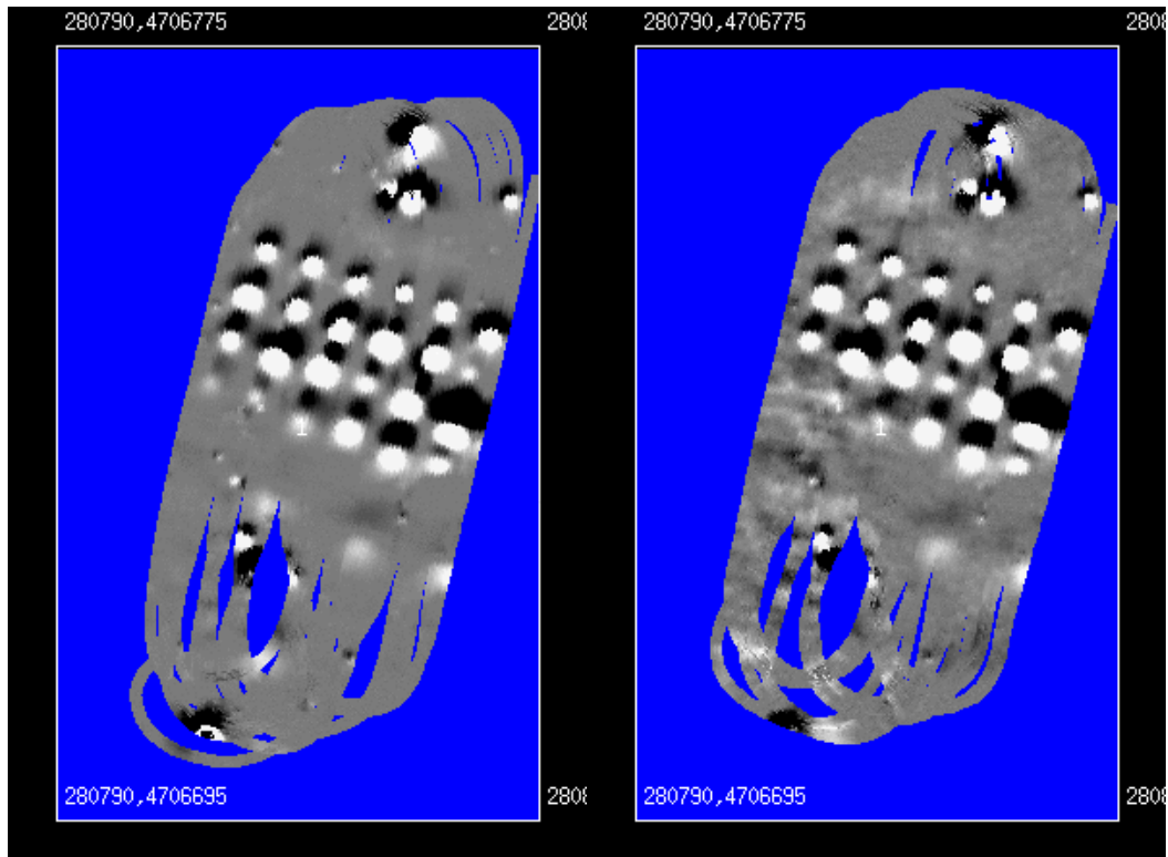
Figure 3: Data taken with steel John Deere Gator tow vehicle showing “cloudy” artifacts due to pitch and roll over rough terrain. Left image is with sensors 20 feet back, right image is with sensors 10 feet back. Both images are de-median filtered and shown at \pm 50 nT. The terrain at the northern and southwestern edge of the Devens site is rough, causing vehicle pitch and roll that changes the magnetic signature seen at the sensors. The de-median filter takes out the bulk signature at both sensor separations, but with the sensors at 10’ the effects from pitch and roll become substantial and are not taken out by the filter.
