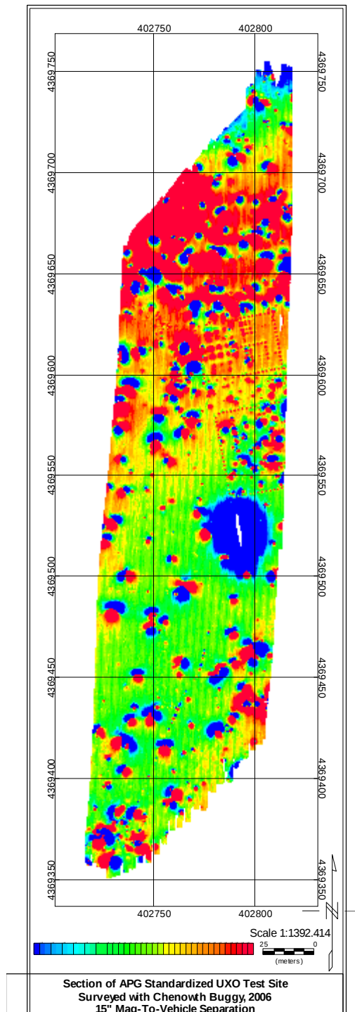
Figure 10: APG Site Legacy Area Section Surveyed in 2006 with Chenoweth Buggy, Mags 15' Back, Uncorrected
