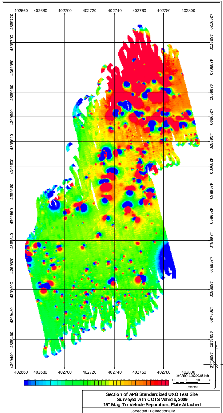
Figure 15: Legacy Area Surveyed with COTS Vehicle, Mags 15' Back, Skidplate Attached, with Bidirectional Correction
