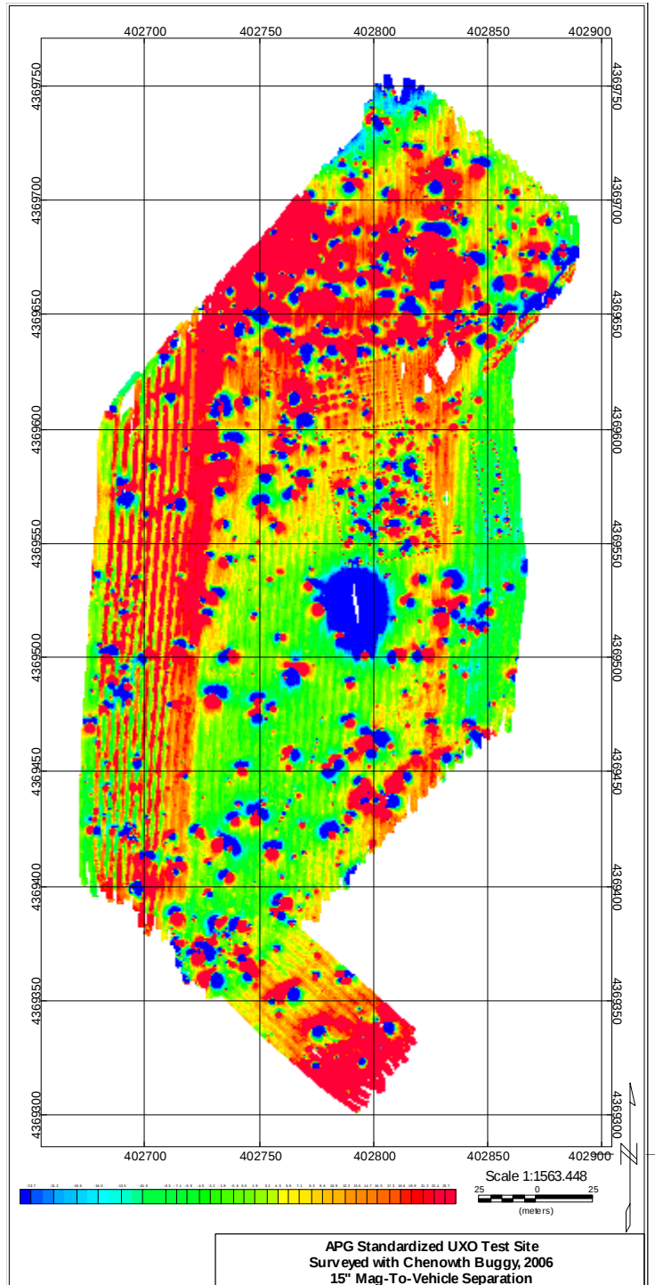
Figure 9: APG Site Surveyed in 2006 with Chenoweth Buggy, Mags 15' Back, Uncorrected
