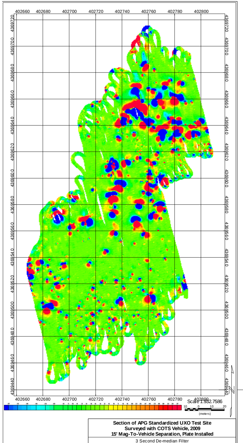
Figure 22: Legacy Area Surveyed with COTS Vehicle, Mags 15' Back, Skidplate Installed, with 3 Second De-median Filter Correction
