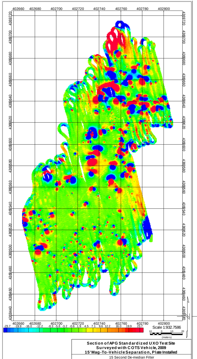
Figure 34: Legacy Area Surveyed with COTS Vehicle, Mags 15' Back, Skidplate Installed, with 15 Second De-median Filter Correction
