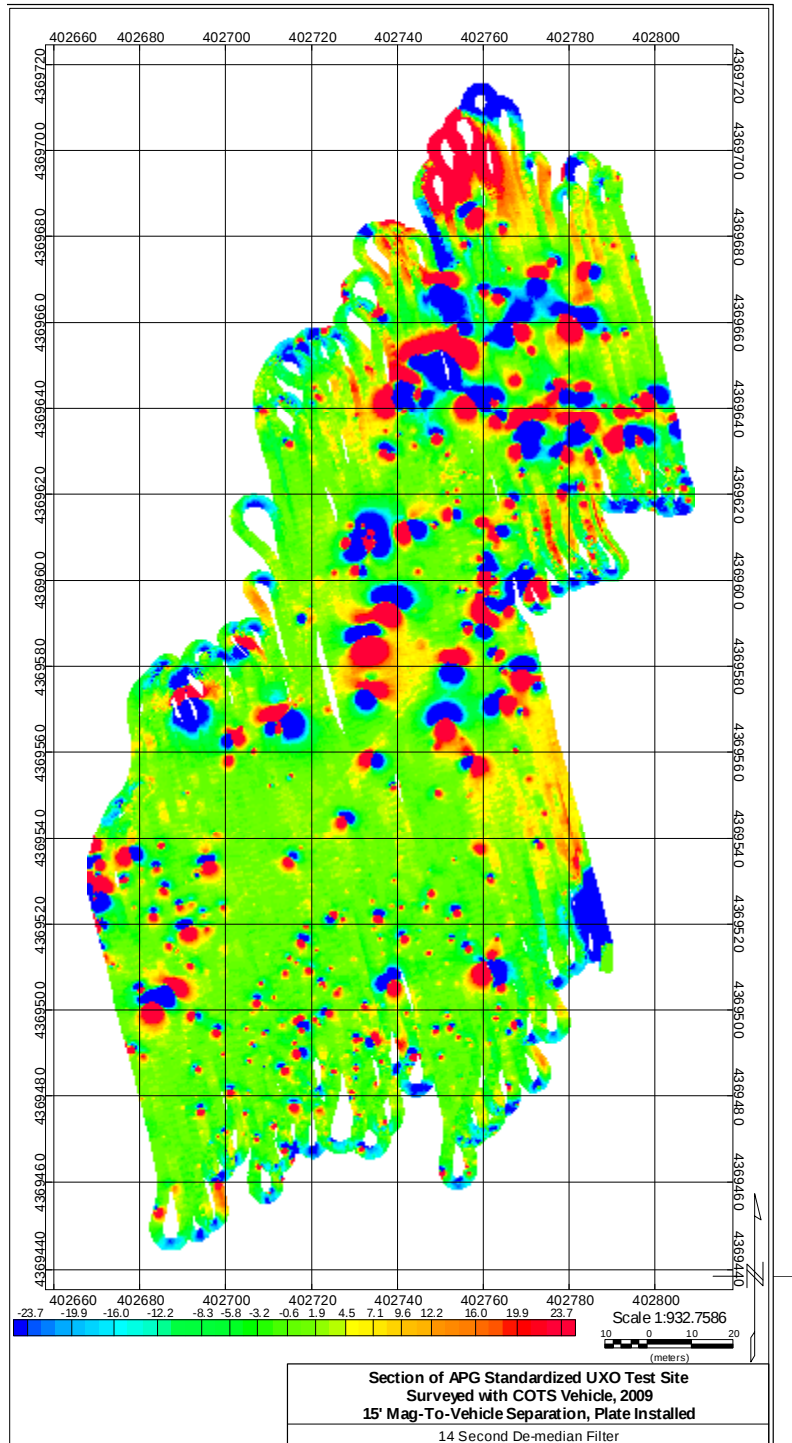
Figure 33: Legacy Area Surveyed with COTS Vehicle, Mags 15' Back, Skidplate Installed, with 14 Second De-median Filter Correction
