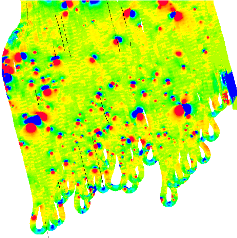
Figure 39: Blowup to show washboard pattern
