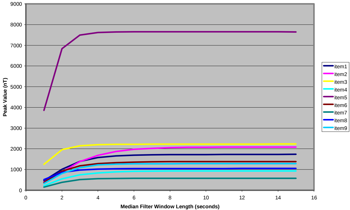
Figure 35: Nine Objects, Anomaly Peak Amplitude as a Function of Median Filter Window Length
