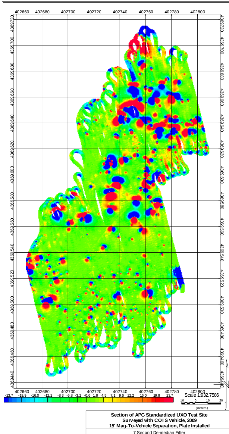
Figure 26: Legacy Area Surveyed with COTS Vehicle, Mags 15' Back, Skidplate Installed, with 7 Second De-median Filter Correction
