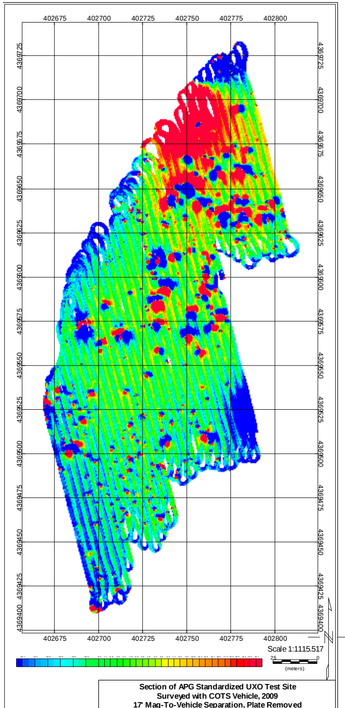
Figure 17: Legacy Area Surveyed with COTS Vehicle, Mags 17' Back, Skidplate Removed, Uncorrected
