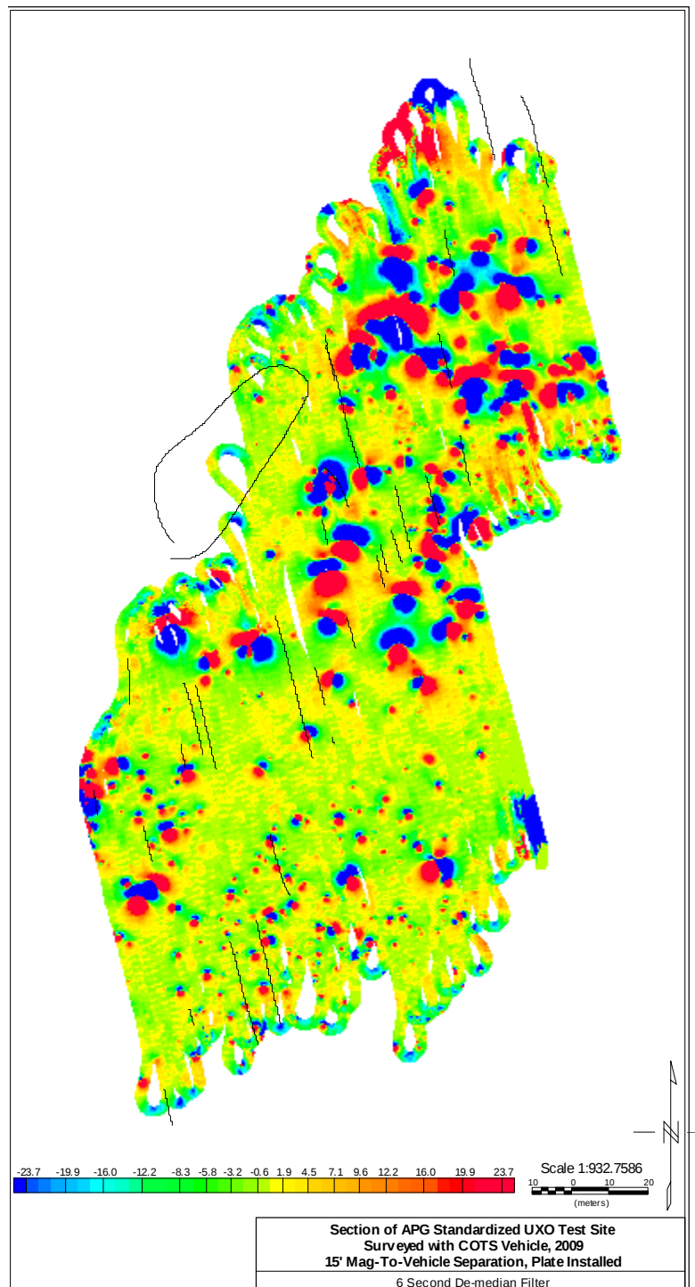
Figure 38: Legacy area with rough areas shown as black lines, color scale pushed to show washboard pattern
