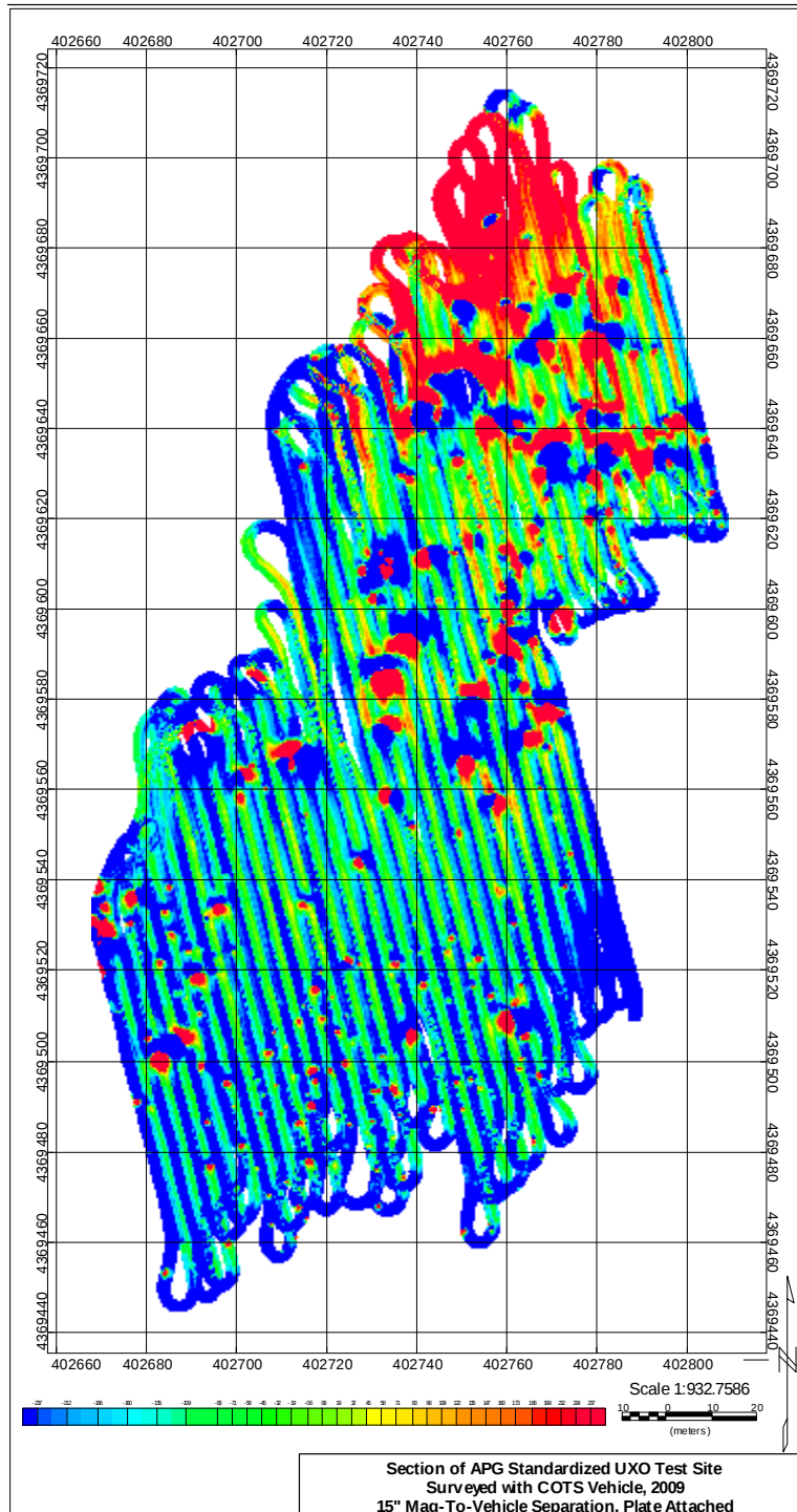
Figure 14: Legacy Area Surveyed with COTS Vehicle, Mags 15' Back, Skidplate Attached, Uncorrected
