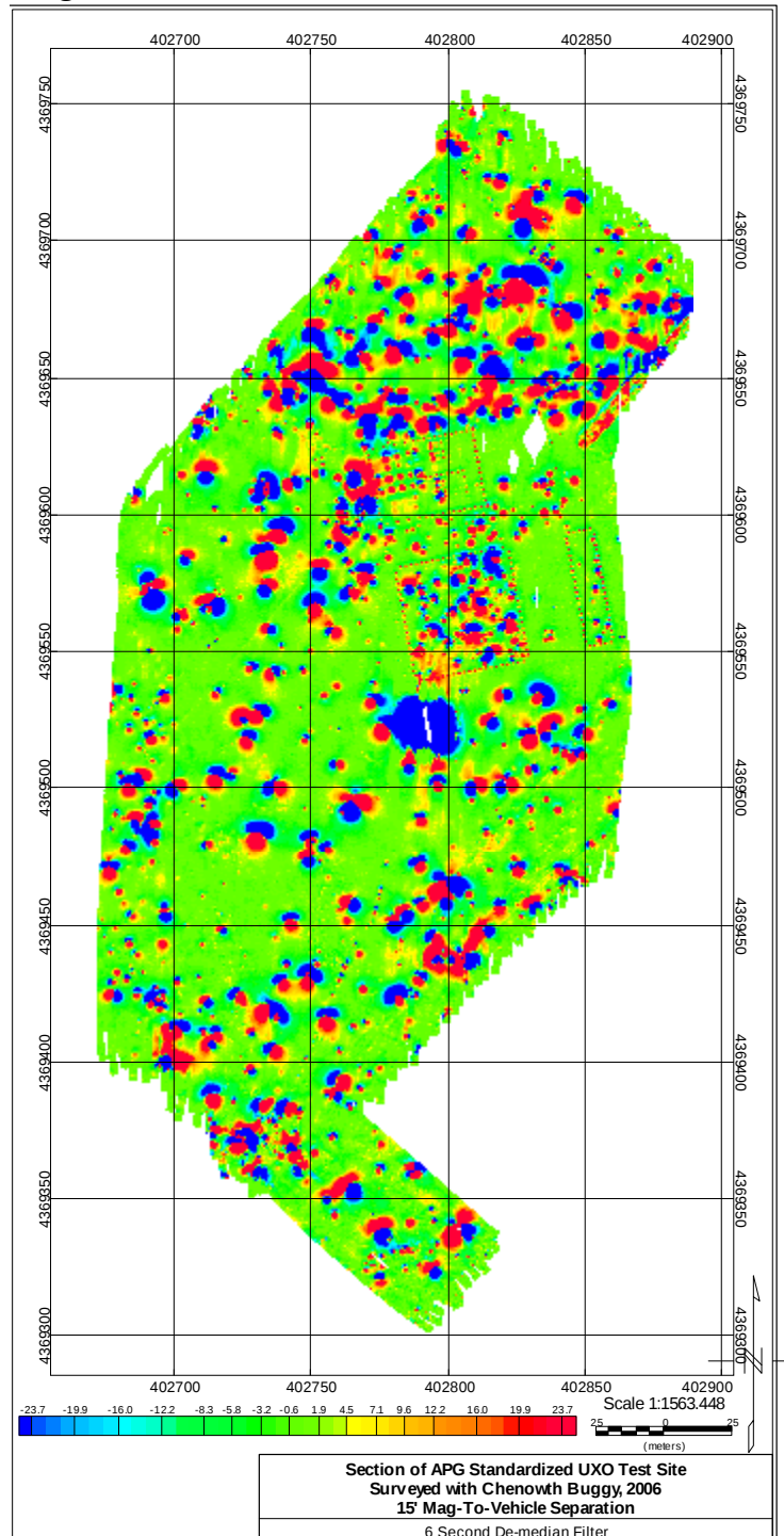
Figure 13: APG Site Legacy Area Plus Adjacent Section Surveyed in 2006 with Chenoweth Buggy, Mags 15' Back, with De-median Correction
