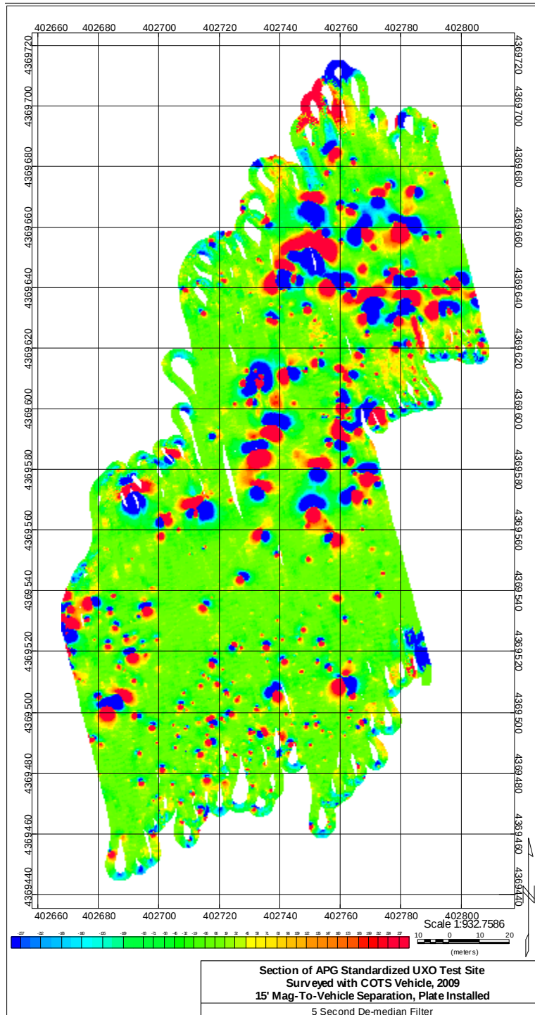
Figure 24: Legacy Area Surveyed with COTS Vehicle, Mags 15' Back, Skidplate Installed, with 5 Second De-median Filter Correction
