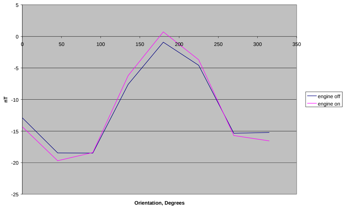
Figure 5: Octant Test, Mag 15' Behind Vehicle, Skidplate Removed
