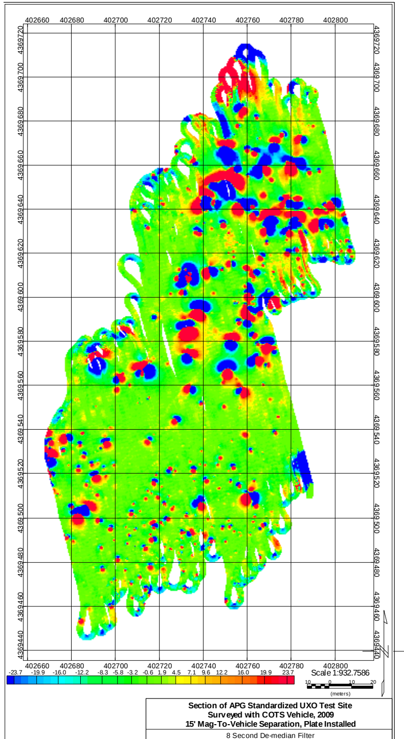
Figure 27: Legacy Area Surveyed with COTS Vehicle, Mags 15' Back, Skidplate Installed, with 8 Second De-median Filter Correction
