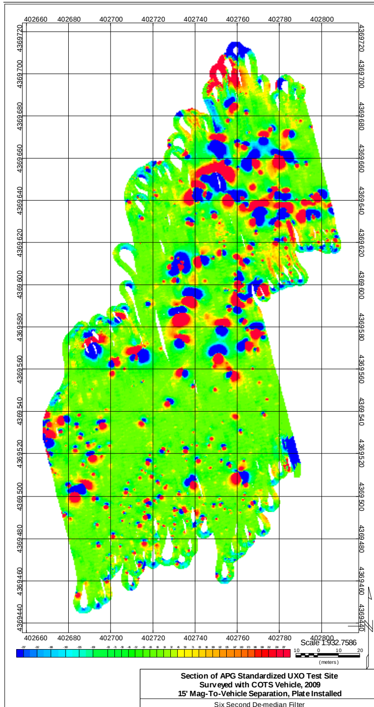
Figure 16: Legacy Area Surveyed with COTS Vehicle, Mags 15' Back, Skidplate Installed, with De-median Filter Correction
