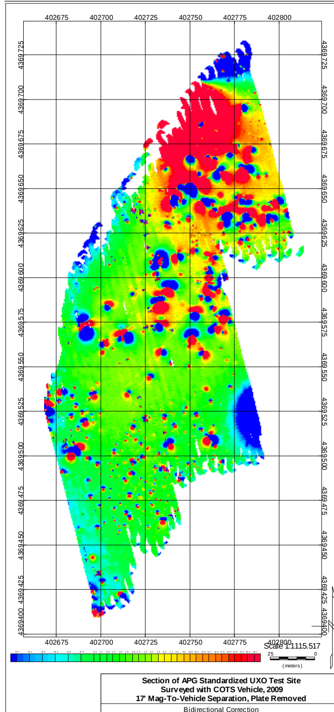
Figure 18: Legacy Area Surveyed with COTS Vehicle, Mags 17' Back, Skidplate Removed, with Bidirectional Correction
