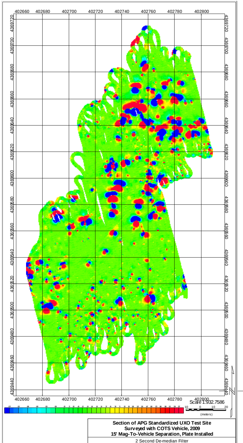
Figure 21: Legacy Area Surveyed with COTS Vehicle, Mags 15' Back, Skidplate Installed, with 2 Second De-median Filter Correction
