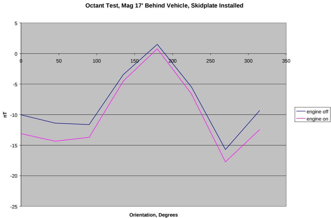
Figure 8: Octant Test, Mag 17' Behind Vehicle, Skidplate Installed
