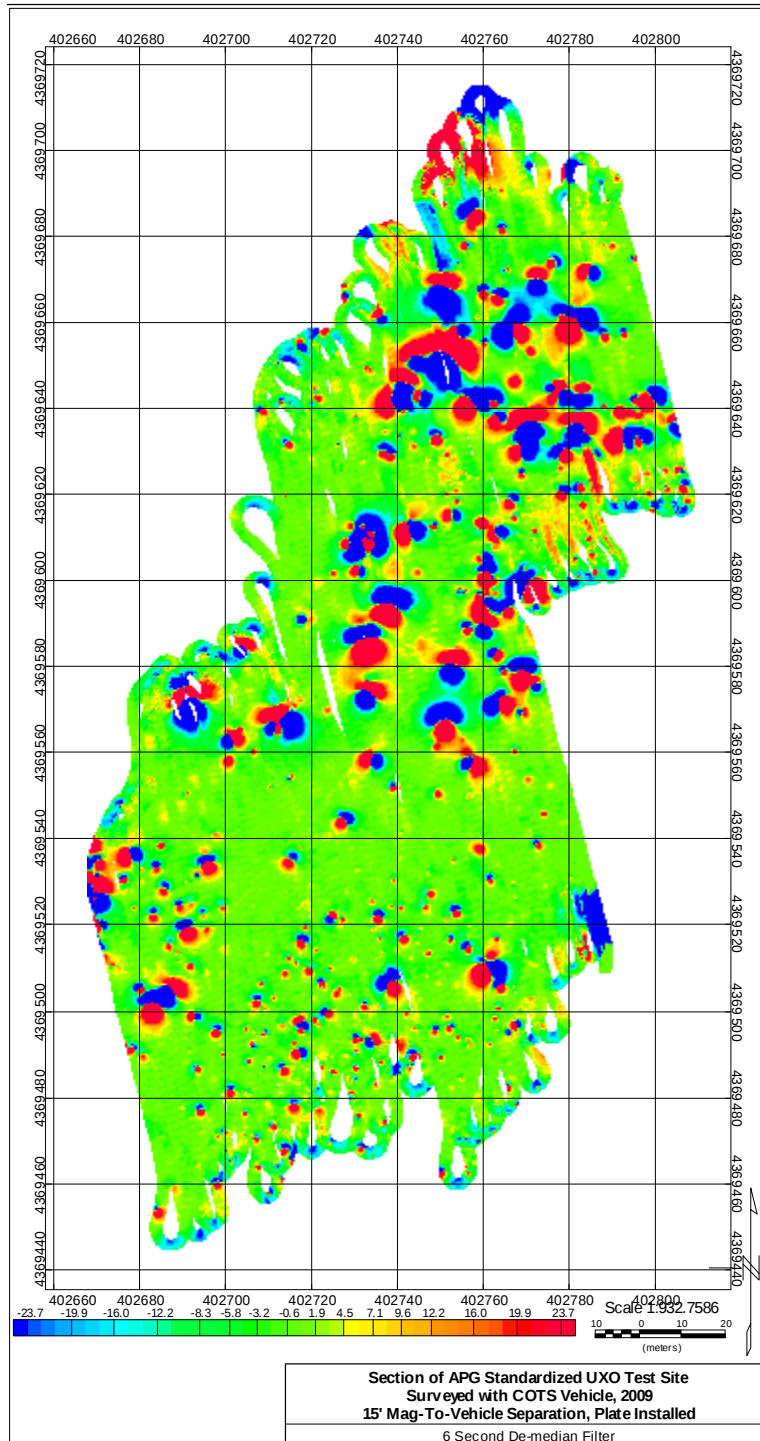
Figure 25: Legacy Area Surveyed with COTS Vehicle, Mags 15' Back, Skidplate Installed, with 6 Second De-median Filter Correction
