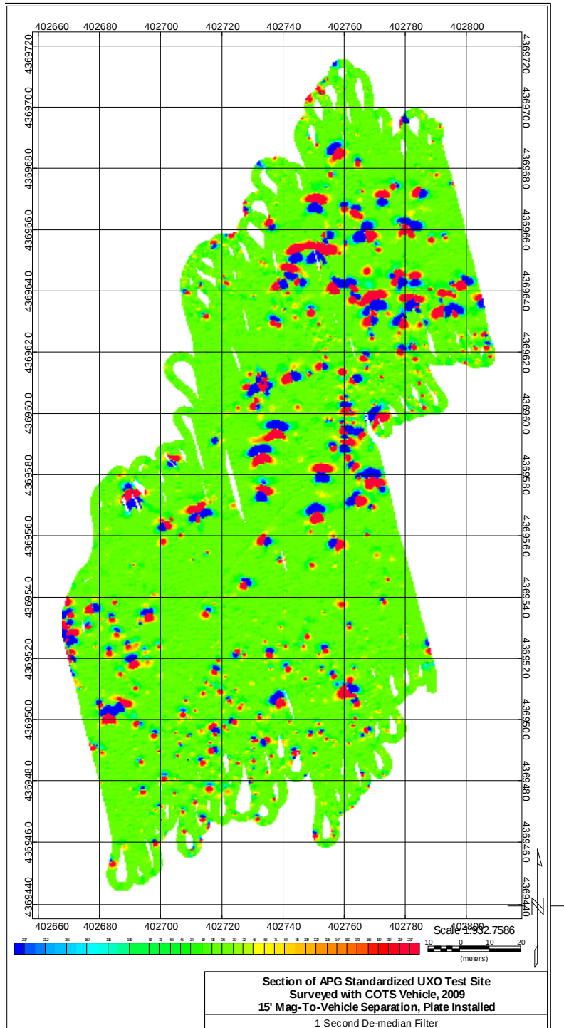
Figure 20: Legacy Area Surveyed with COTS Vehicle, Mags 15' Back, Skidplate Installed, with 1 Second De-median Filter Correction
