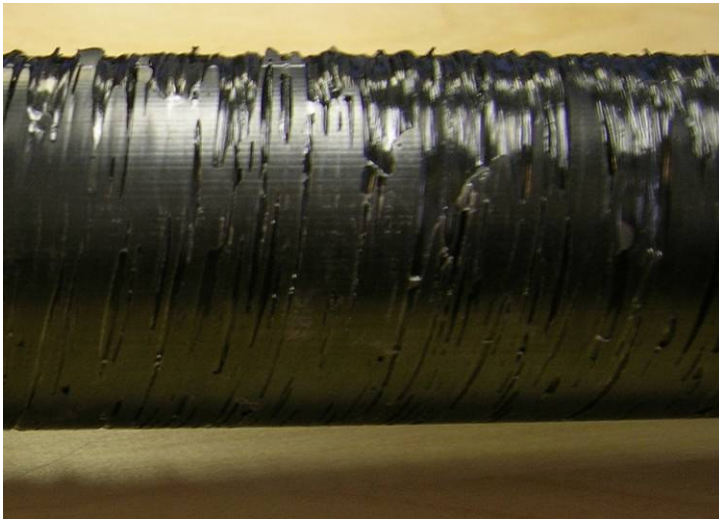
Fig. 8. Tube wound with conventional prepreg on an undersized mandrel, and then cured in a female mold. Note severe hammocking.
