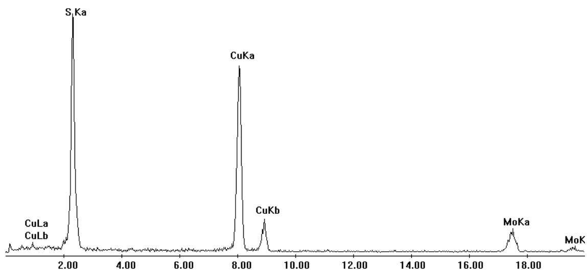
Figure 2. EDX spectra of MoS 2 nanoparticles (distinctive peaks of Mo and S of molybdenum sulfide pattern, Cu signal is from TEM grid)
