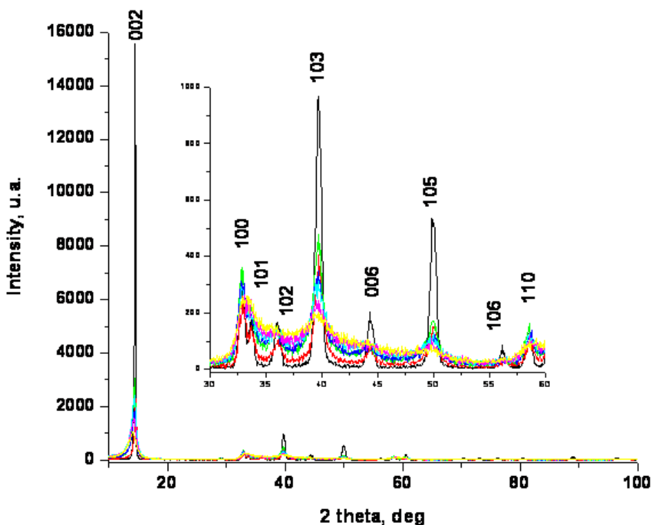
Figure 3. Powder XRD of MoS 2 samples
