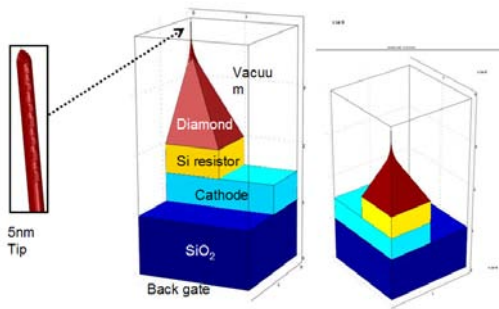
Figure 4 Simulation cell for the diamond bg-FEA. Thicknesses: SiO 2 -0.5μm, cathode-0.5μm, ballast resistor- 0.5μm. Entire cathode assumed conductive.
