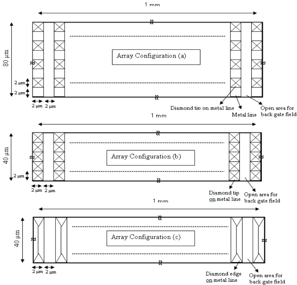
Figure 3: Proposed field emission array configurations
