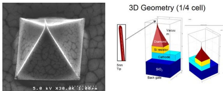
Fig.1 Electrostatic simulation of back-gate cathodes with diamond tip (right) arrays predicts current modulation of between 10^2 - 10^3 to achieve program goal of 750\text{ A}/\text{cm}^2 .
