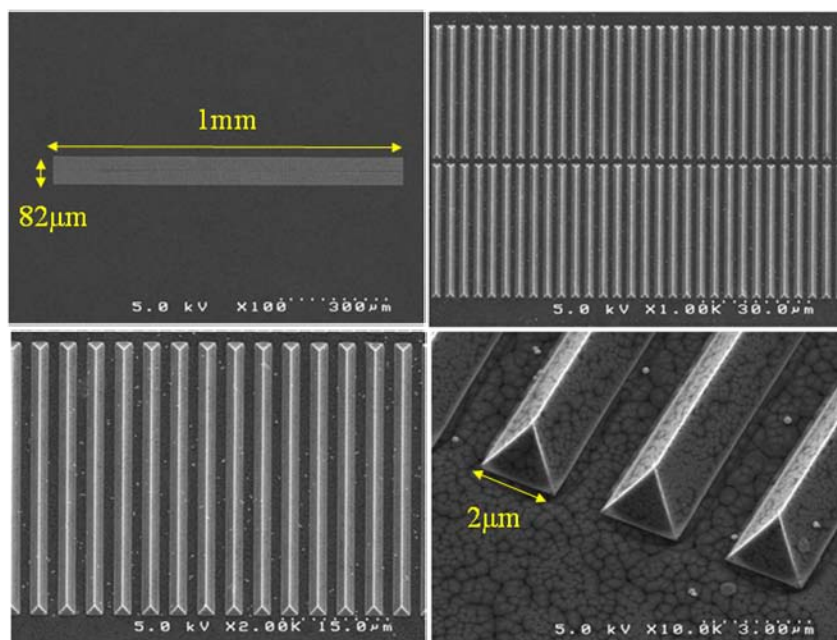
Figure 14: SEM micrograph of fabricated diamond edge FEAs.
