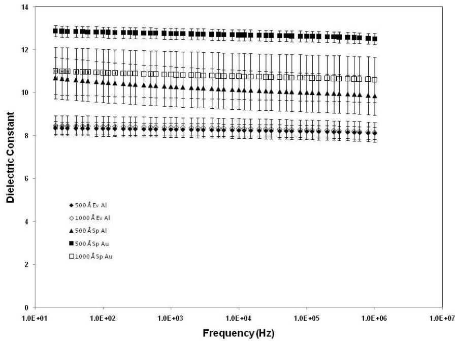
Figure 4. Dielectric constant vs. frequency for AlON films with various electrode metals and deposition methods.
