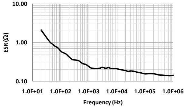
Figure 7: ESR versus frequency of the FPE capacitor.
