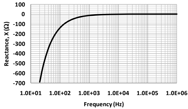
Figure 8: Reactance versus frequency of the FPE capacitor.
