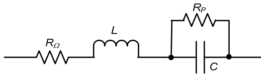
Figure 1. Equivalent circuit model of a capacitor.
