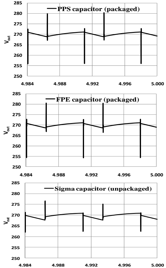
Figure 12. Output Voltages of FPE, and PPS packaged capacitors and Sigma capacitor for a 100 V/270 V, 10 kW, 75 kHz interleaved DC-DC converter. 4 -10 uF capacitors were connected in parallel for FPE and PPS Figures. For Sigma capacitors, a total of 12 capacitors are used. (3 in series and 4 in parallel).
