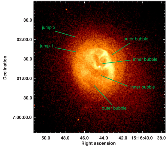
Figure 1. 0′.49 Gaussian-smoothed Chandra ACIS-S3 image of the central 3/4×3/4 region of Abell 2052. The image has been corrected for background and exposure. Several bubbles related to AGN outbursts are indicated, as well as discontinuities in the surface brightness surrounding the cluster center. These discontinuities are modeled as density jumps and are labeled “jump 1” and “jump 2.”
