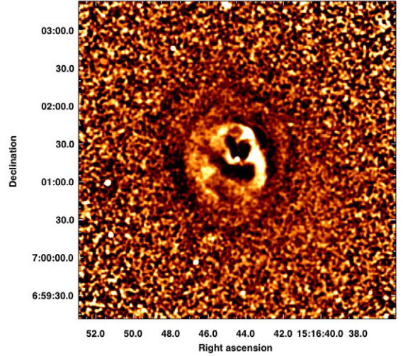
Figure 2. Unsharp-masked Chandra ACIS-S3 image of the central 4/2×4/2 region of Abell 2052.
