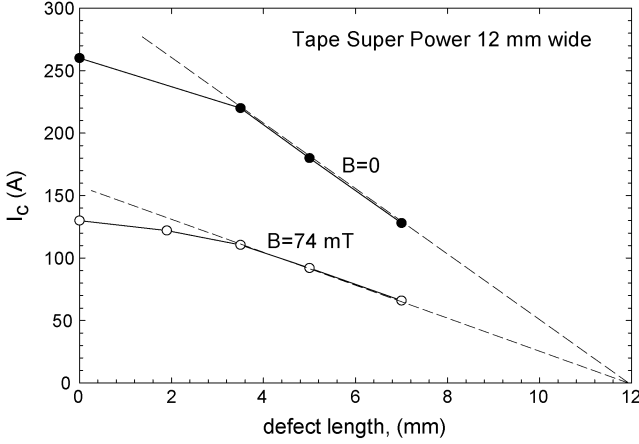
Fig. 5. Critical current I_c defined by 1 \mu\text{V}/\text{cm} at zero applied field and B = 74 \text{ mT} as a function of the defect length.
