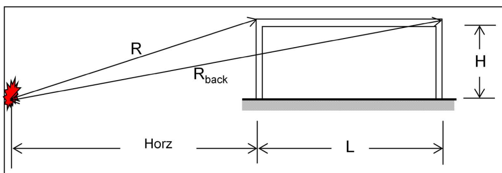
Figure 10 Factors for predicting blast loading to roofs
