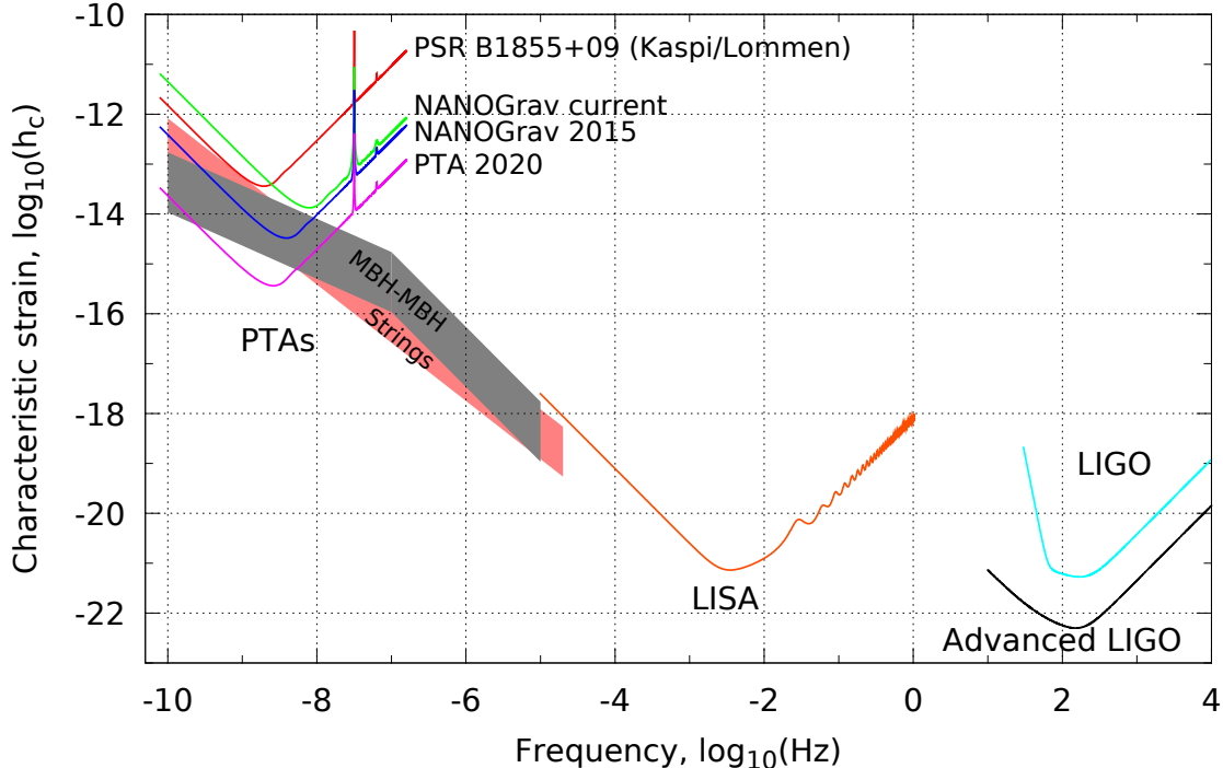
Figure 1: Comparison of current and planned GW detectors, showing characteristic strain ( h_c ) sensitivity versus frequency along with expected source strengths. The Laser Interferometer Gravitational Wave Observatory (LIGO), the Laser Interferometer Space Antenna (LISA) and PTAs occupy complementary parts of the GW spectrum.
