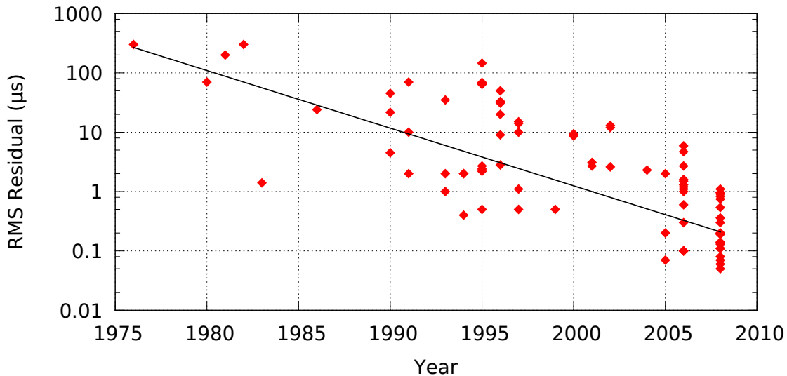
Figure 3: Published RMS pulsar timing residuals versus time, showing exponential improvement (Demorest & Jenet, 2009) which positions us to detect GWs within the next decade.
