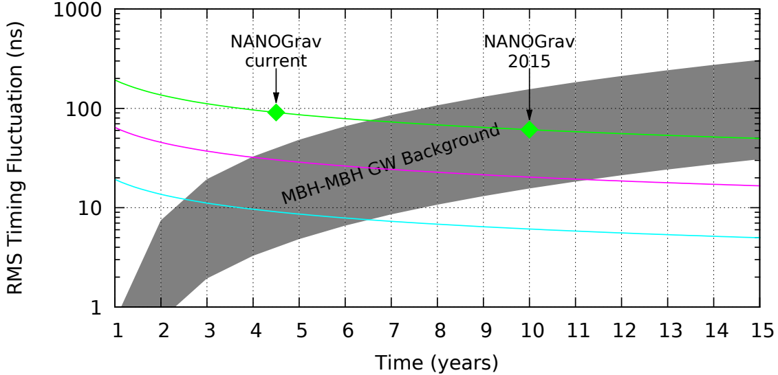
Figure 2: PTA sensitivity versus times for several scenarios: The current NANOGrav observing program, and potential future PTAs of 3 and 10 times better GW sensitivity. The shaded area shows the expected amplitude range of the MBH-MBH GW signal (see §2.1).
