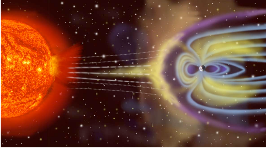
Figure 1. Illustration of the interaction between the Sun and Earth's magnetosphere ( not to scale ). In this example, an eruption from the Sun has reached the Earth, compressed the magnetosphere, and injected energetic particles. Credit: NASA
