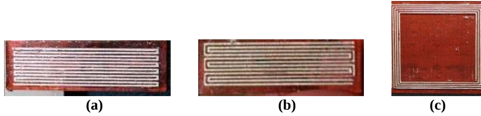
Figure 7. Cured ink SL RLC test models; (a) Serpentine design increases resistance over length of ink line to allow for measurable data; (b) Parallel serpentine design increases capacitance over length of ink line to allow for measurable data; (c) Loop design allows for the inductance of two adjacent ink lines to add while minimizing the attenuation of their magnetic field.
