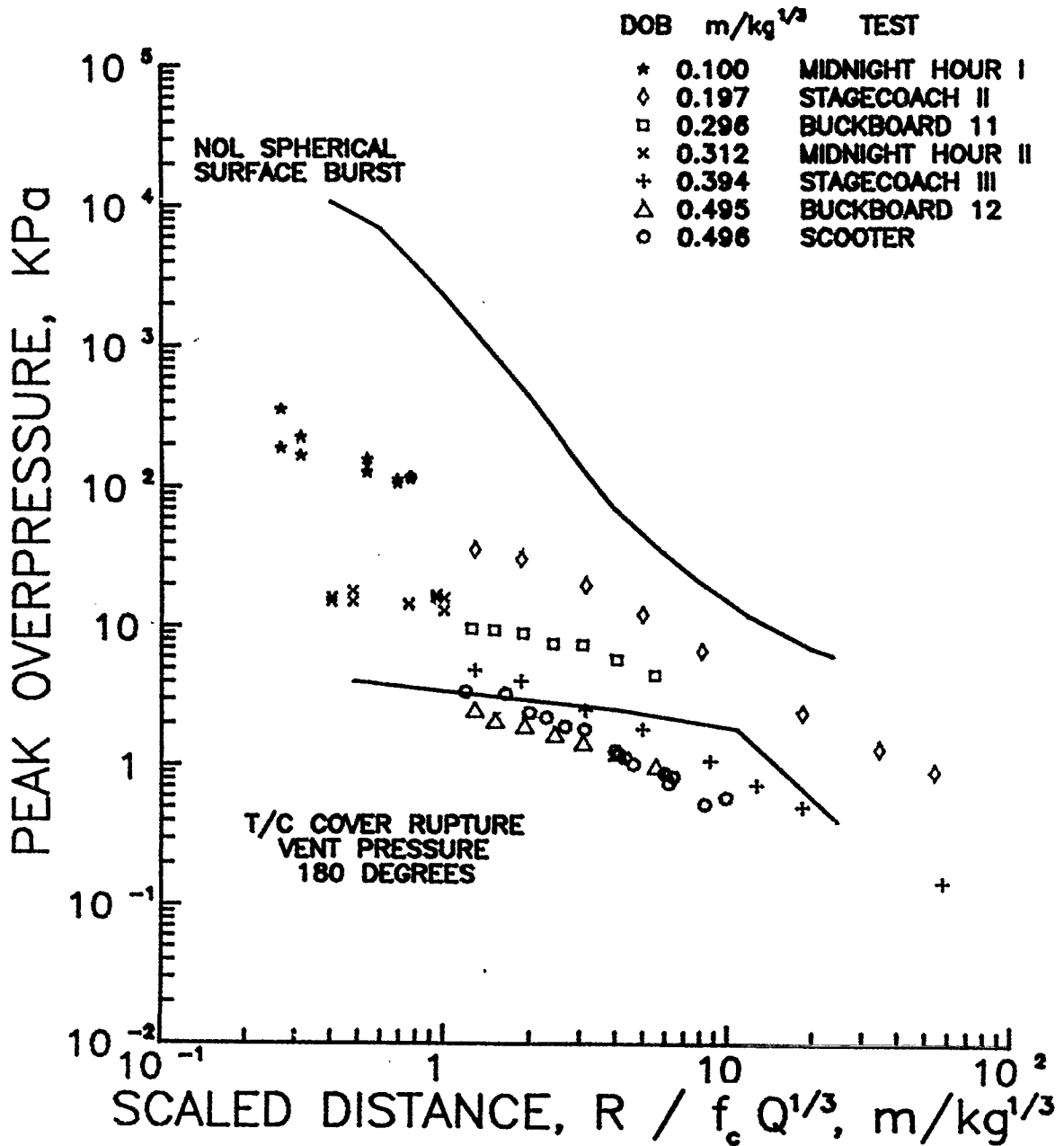
Figure 4. Comparison of vented airblast overpressure data from fully-coupled, buried detonations in desert alluvium with the NOL calculated pressure for spherical surface bursts and measured vent pressures from the decoupled Tunnel/Chamber test.
