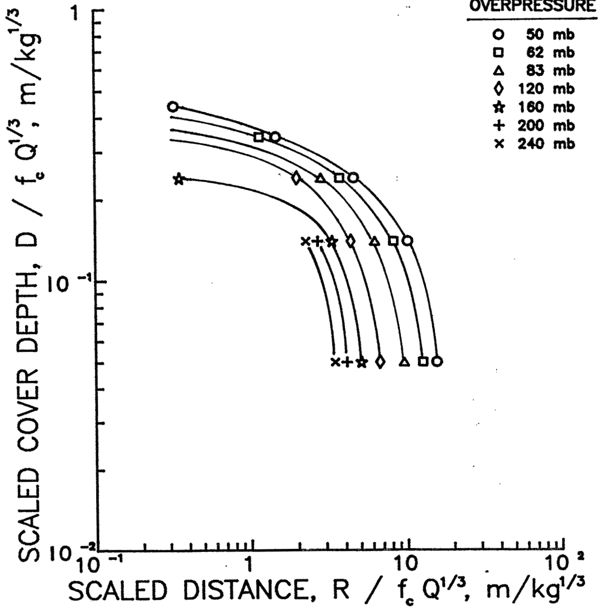
Figure 7. Airblast overpressure contours as a function of scaled cover depth and scaled horizontal distance from detonations in underground munitions storage chambers.
