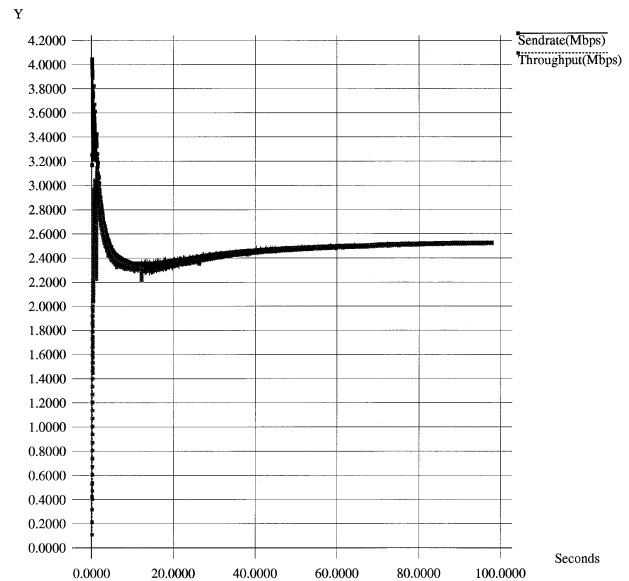
Fig. 3. Stabilization at 2.5 Mb/s throughput under background large file ftp at host with web browsing.
