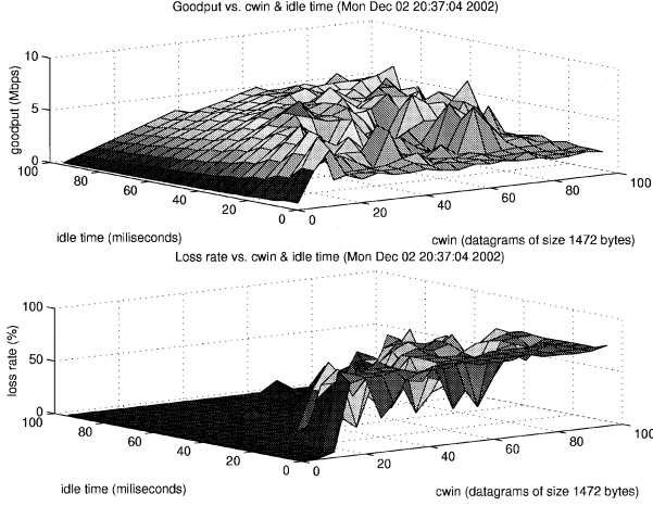
Fig. 1. Internet measurements with sending rate along horizontal plane, and throughput and loss rate along vertical axes in top and bottom plots, respectively.
