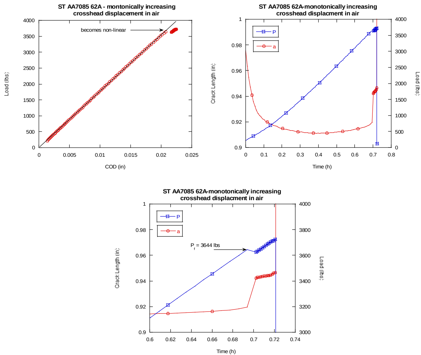
Figure 1 - Test results for ST specimen 62A that was tested in air at a monotonically increasing crosshead displacement.
