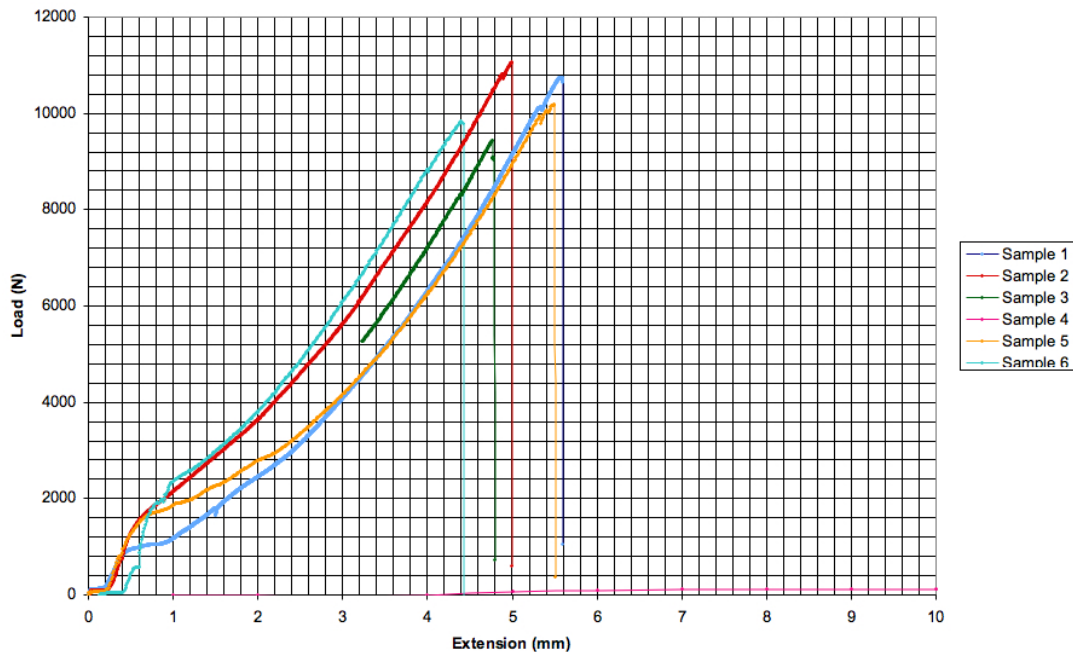
Fig. 21 shear load vs extension for thermoset FM300K
