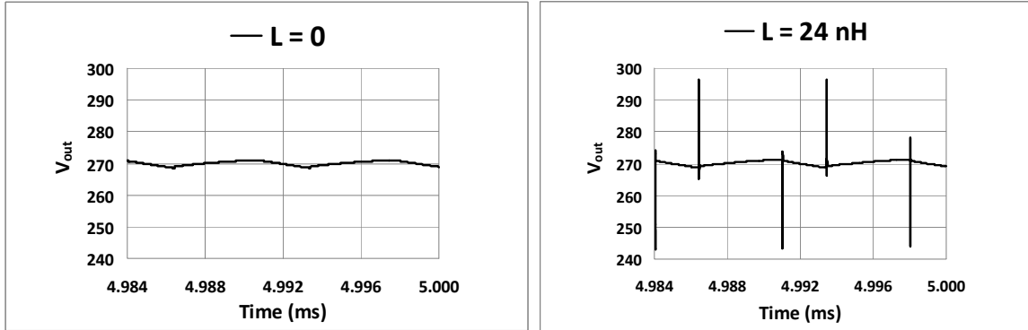
Figure 11. Effects of ESL on output voltage ripple of a 100 V/270 V, 10 kW, 75 kHz interleaved dc/dc converter. 4 -10 \mu F capacitors were connected in parallel. ESR of each capacitor was assumed to be 30 m \Omega . (Left Figure: ESL=0 nH, Right Figure: ESL=24 nH)
