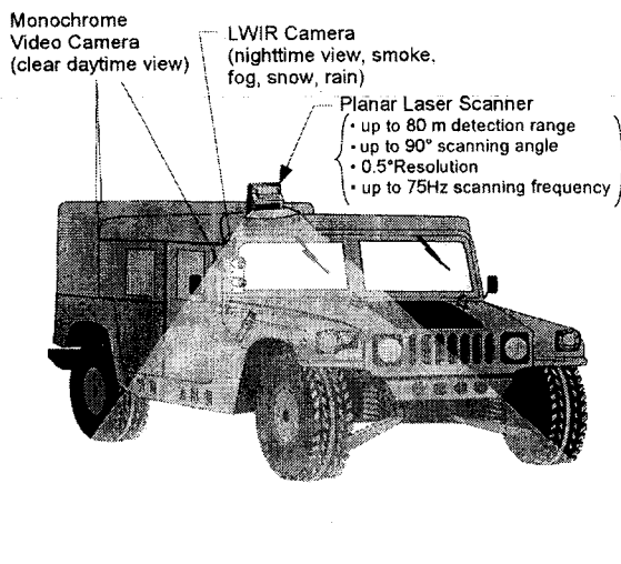
Figure 2: Video and LWIR Cameras potential Mounting Positions.
