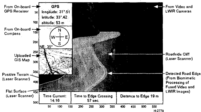
Figure 6: Conceptual Design for the DVI Display
