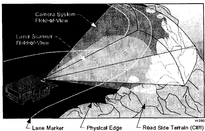
Figure 3: Potential Scanning Range of the Camera System.
