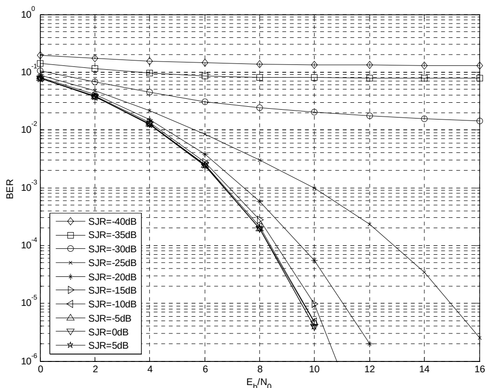
Figure 4: BER performance for uncoded QPSK in MT jamming, for a 1x5MHz system, subject to 175 evenly distributed jamming tones.
