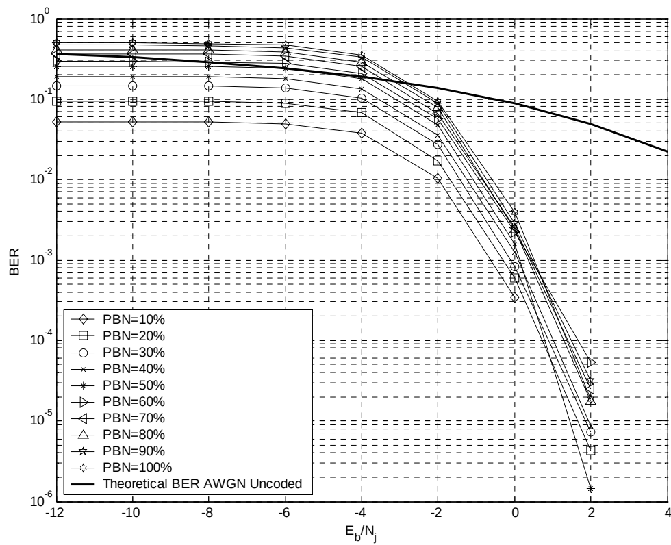
Figure 2: BER performance for rate 1/2 QPSK in PBN jamming, for a 1x5MHz system, with a residual E_b/N_0=10\text{dB} .
