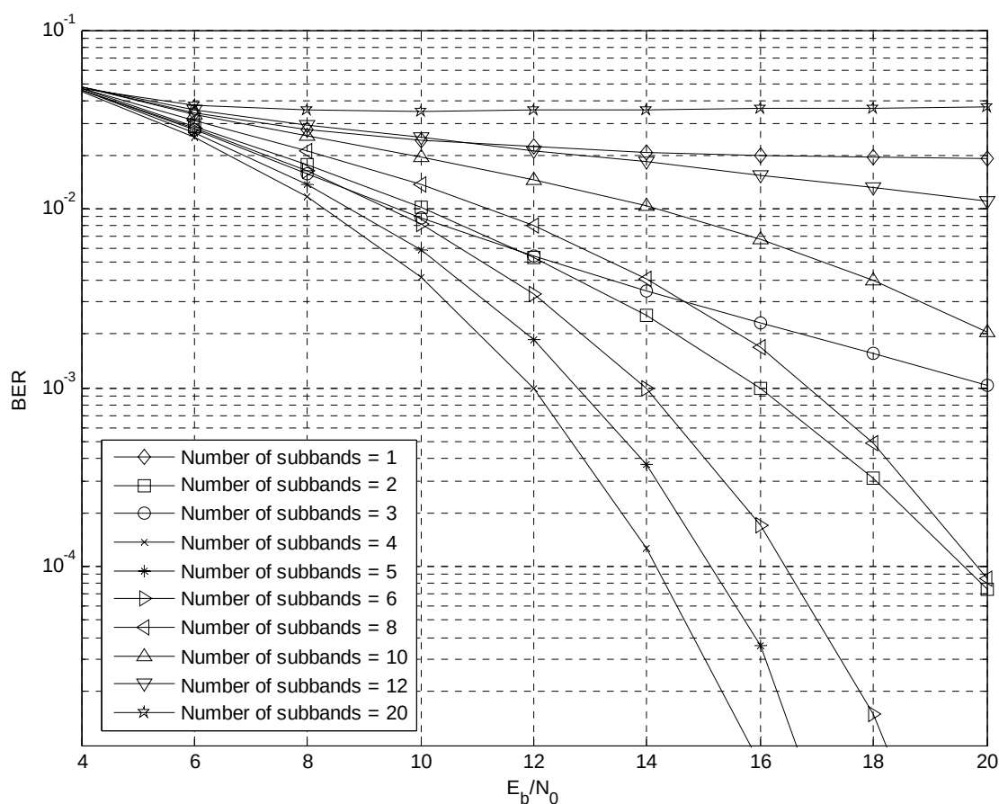
Figure 6: BER performance for uncoded QPSK in MT jamming, for various subbands, subject to 175 evenly distributed jamming tones of SJR=-30dB.
