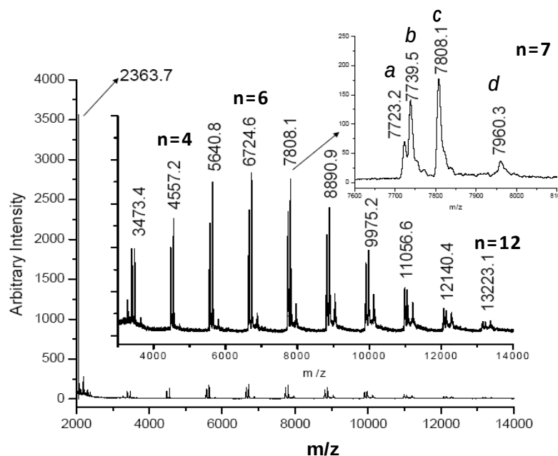
Figure 6. Ethyl isobutyrate Phenyl POSS PMA mass spectrum using 4,4'-dihydroxyoctafluoroazobenzene matrix. Typical series ( a-d ) shown in expansion region of m/z = 7800 .
