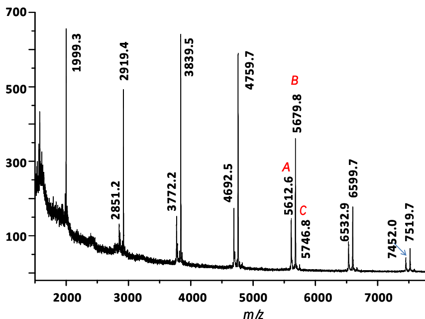
Figure 10. Isobutylnitrile (i-butyl)styrylPOSS MALDI mass spectrum using 4,4'-dihydroxyoctafluoroazobenzene matrix. Labels A, B, And C correspond to 1-3 isobutylnitrile groups.
