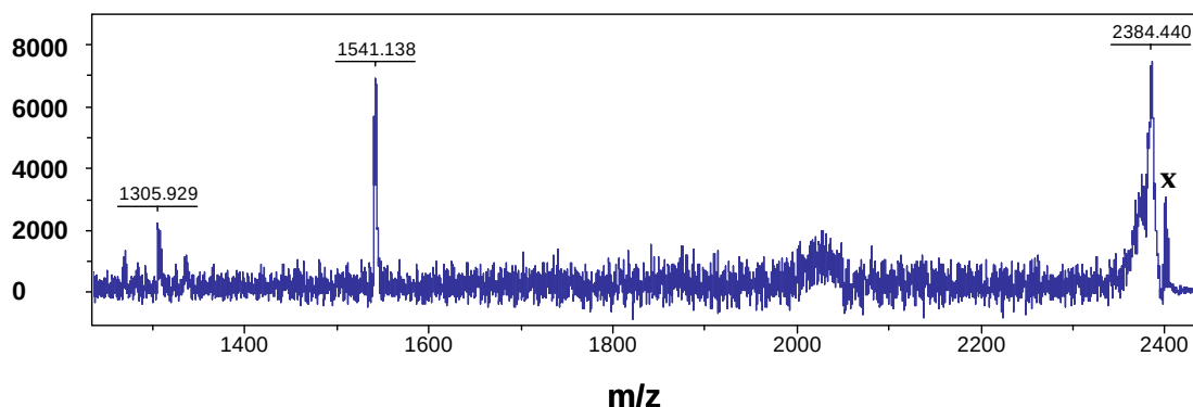
Figure 8. MSMS MALDI spectrum of phthalimido-Isobutyl POSS PMA using 4,4'-dihydroxyoctofluoroazobenzene matrix for the m/z 2397 peak (x).
