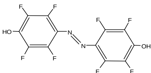
Figure 1. 4,4’-dihydroxyoctafluoroazobenzene matrix.
