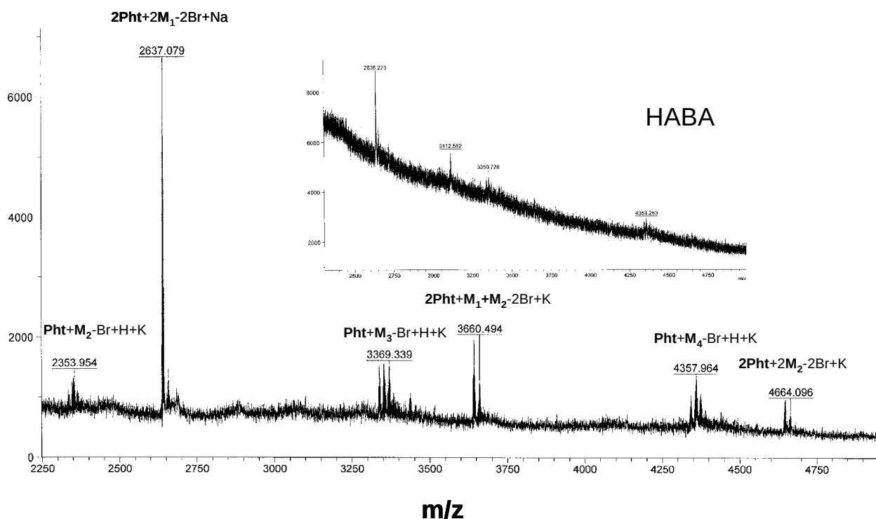
Figure 9. MALDI mass spectra of (Cp) styryl POSS in 4,4'-dihydroxyoctafluoroazobenzene. Inset shows spectrum in HABA matrix.
