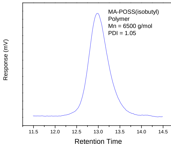
Figure 2. GPC of MA-POSS(isobutyl) polymer.
