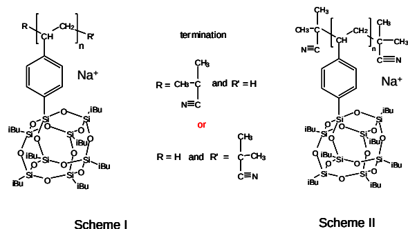
Scheme 4. Free radical termination in i-butyl POSS styryl oligomers. Scheme I: single i-butylnitrile; Scheme II: two i-butylnitrile groups.
