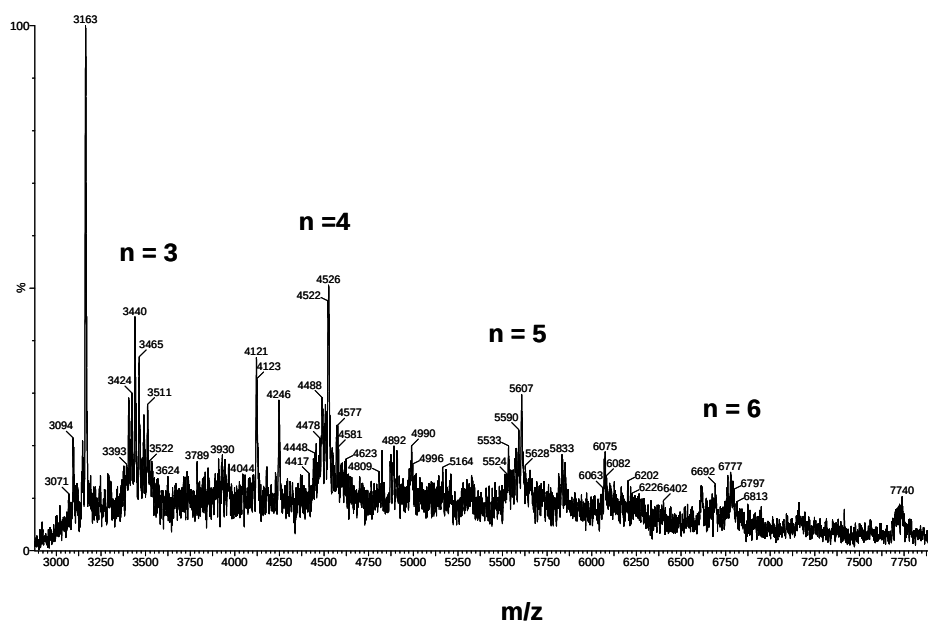
Figure 7. ESI mass spectrum of \text{CH}_3\text{CH}_2\text{OOC}-\text{C}(\text{CH}_3)_2-[(\text{phenyl})_7\text{T}_7\text{propylmethacrylate}]_n . The largest peak in each series up to n = 6 corresponds to protonation of the parent.
