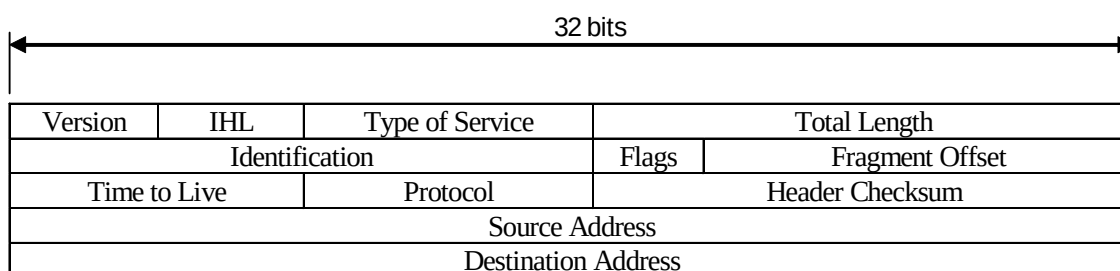
Figure 15: IPv4 packet header
