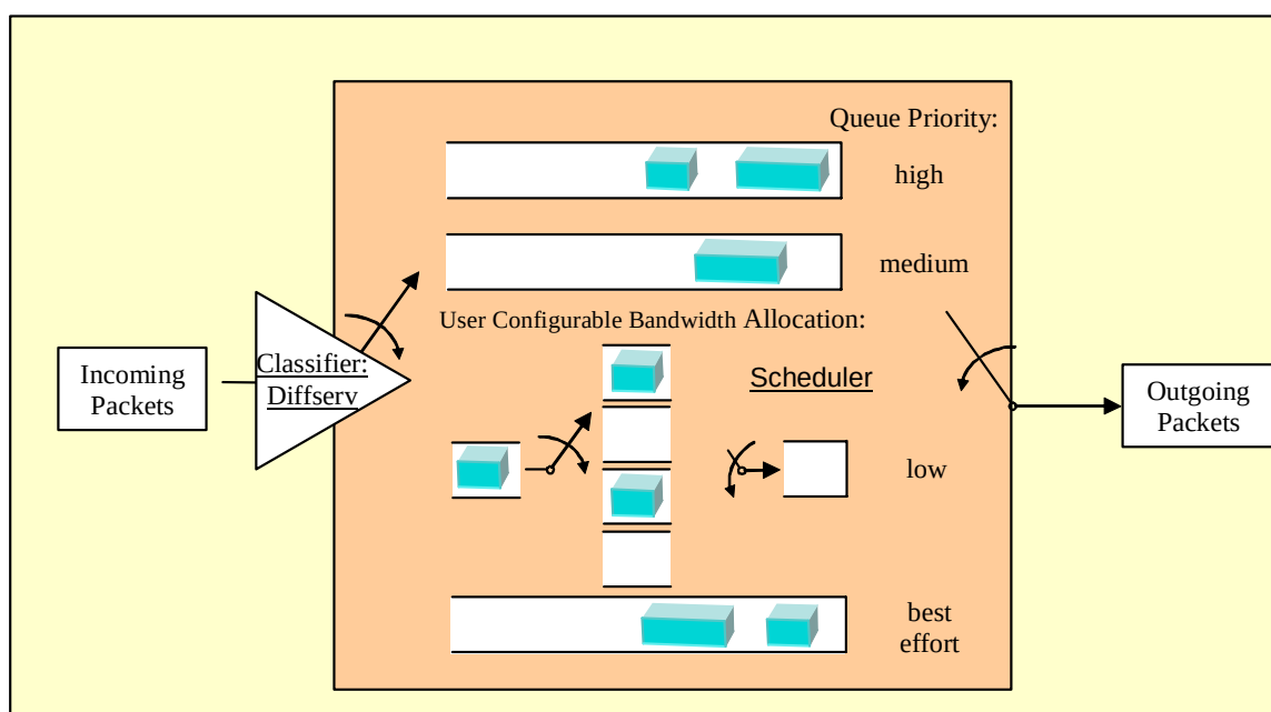
Figure 13: Scheduling and Queuing
