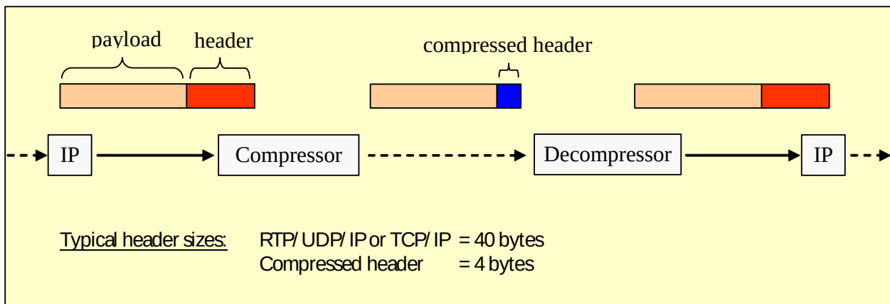
Figure 14: Header compression
