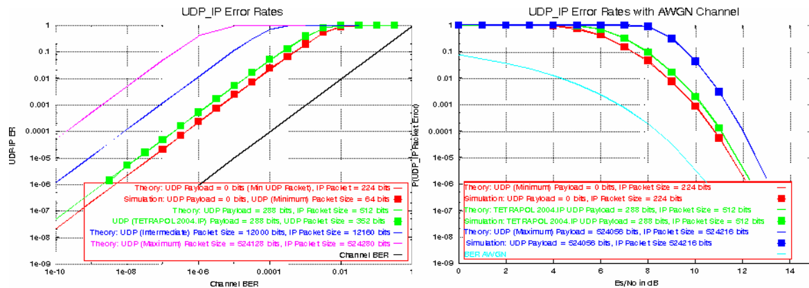
Figure 4: UDP/IP Packet Loss Probability for the BSC (a) and AWGN Channel (b).
