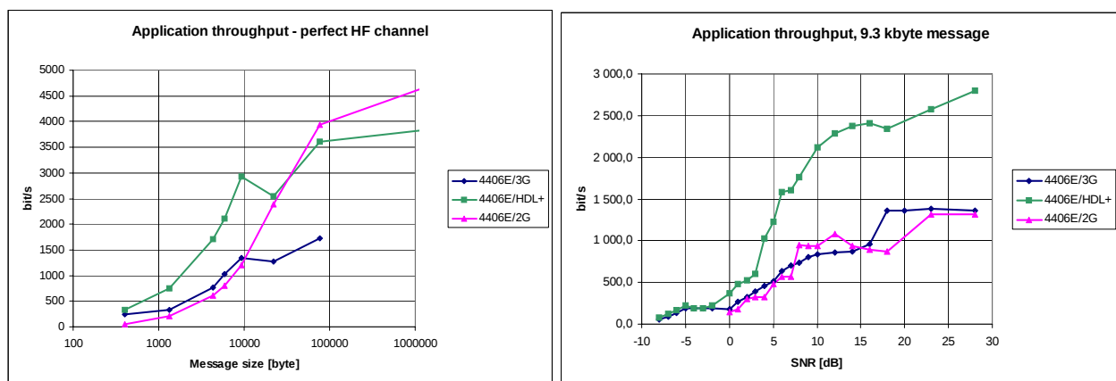
Figure 4: Comparison of throughput vs message size (left) and comparison of throughput vs SNR for a 9.3 kbyte message (right)
