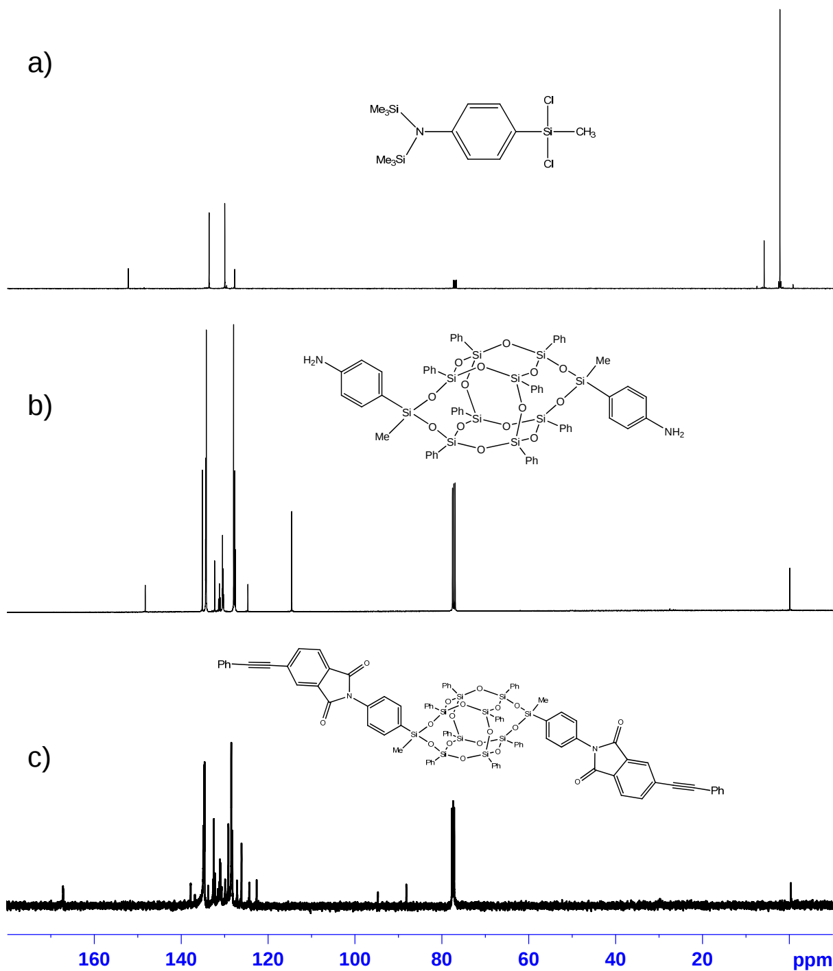
Figure 3. ^{13}\text{C} NMR of (a) (n-trimethylsilyl) _2 -aniline-4-dichloromethylsilane; (b) \text{Ph}_8 bisaniline-POSS (cis and trans isomers); and (c) \text{Ph}_8 bisPEPI-POSS (cis and trans isomers).
