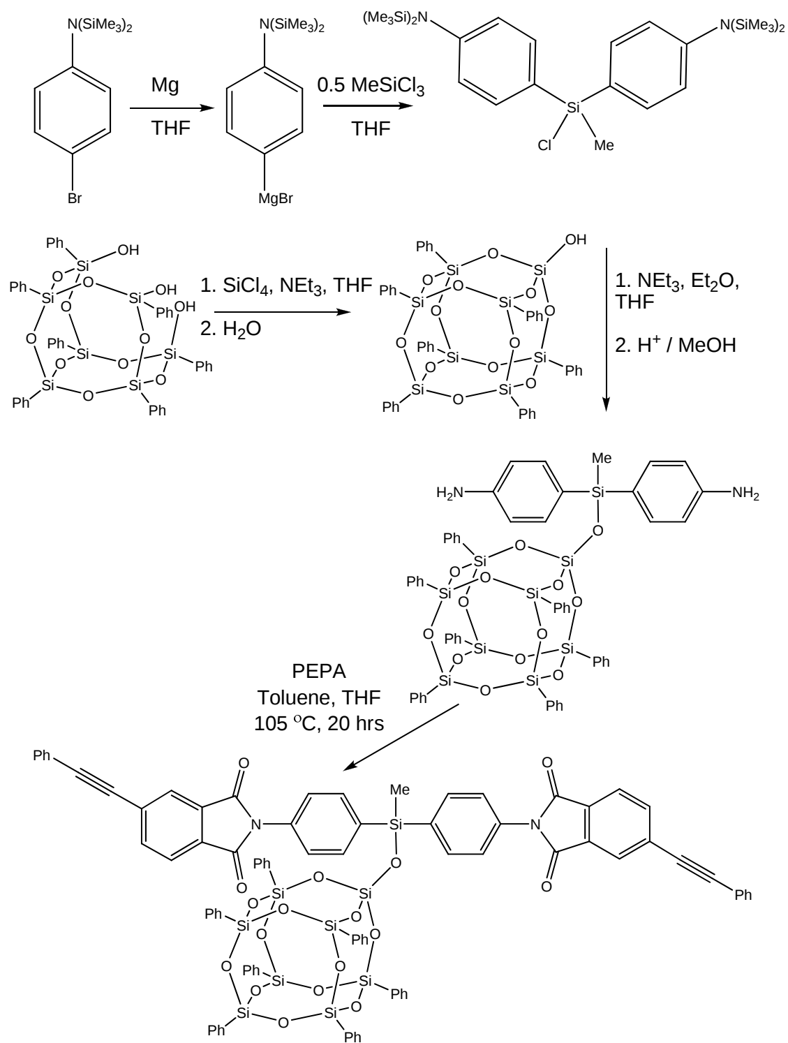
Scheme 2. Synthesis of \text{Ph}_7\text{diPEPI-POSS}
