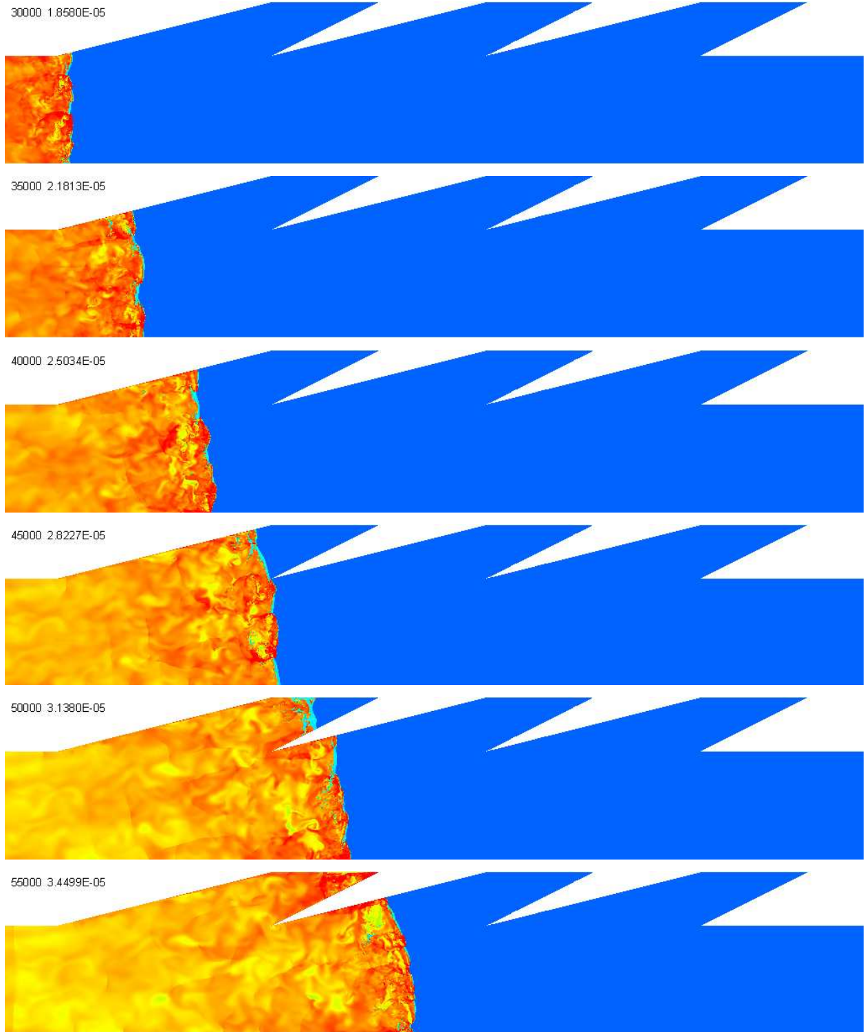
Fig. 2. (continued on next page) Detonation propagation through sawtooth geometry. Timesteps and times in seconds are shown in frame corners. Colors show temperature (see colormap in Fig. 3)
