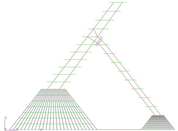
Figure 7 XY View internal structure FE model
