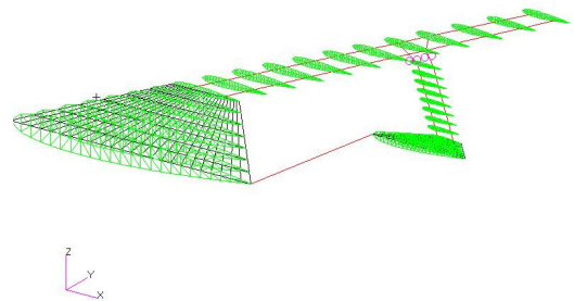
Figure 9 XYZ View internal structure of FE model
