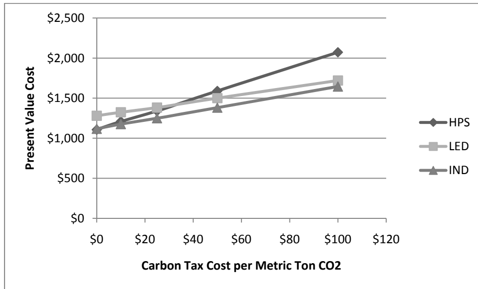
Figure 30. Carbon Emission Offset Cost Sensitivity for Low CO 2 Emission Location (Mt Home AFB)
