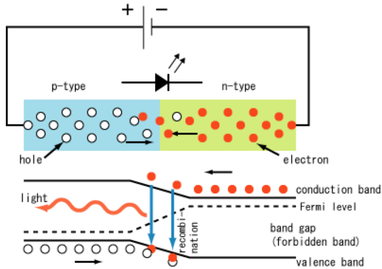
Figure 9. P-N Junction of a Light-Emitting Diode (Wikipedia, 2009)
