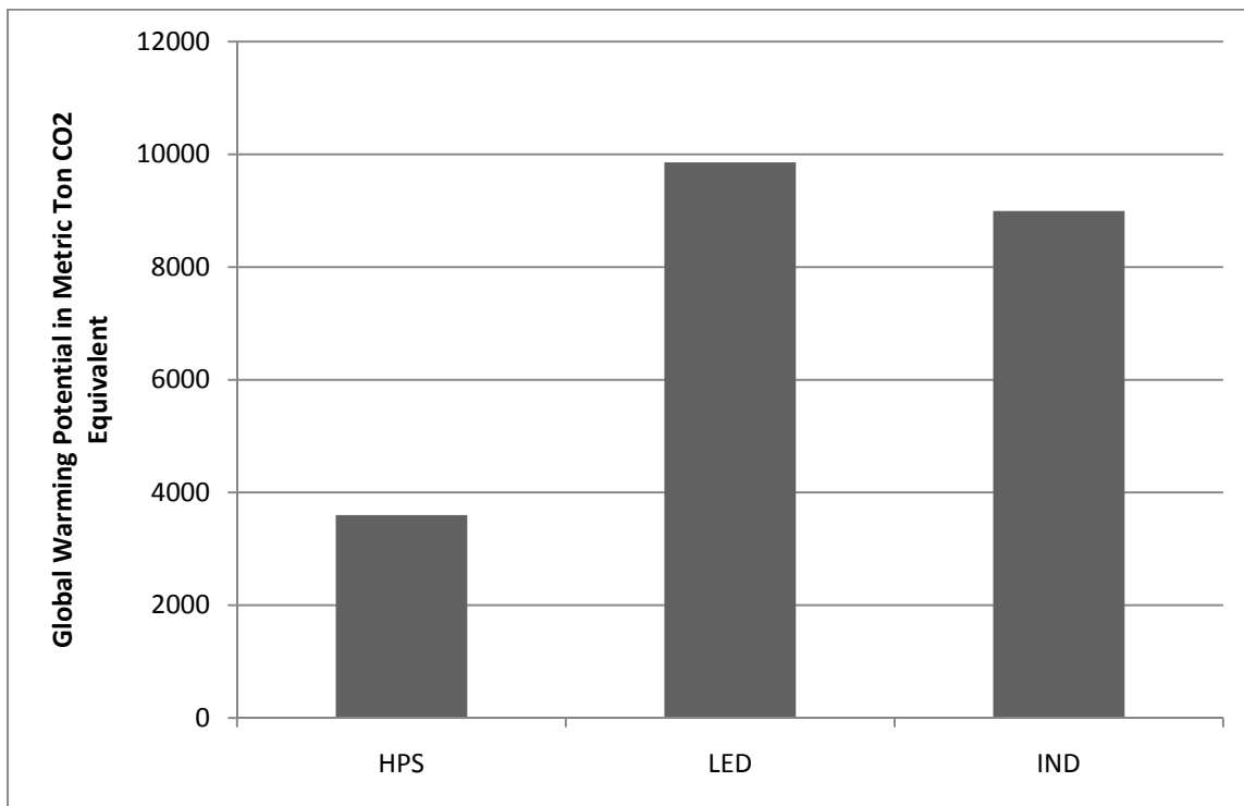
Figure 32. Manufacturing Phase Emissions
