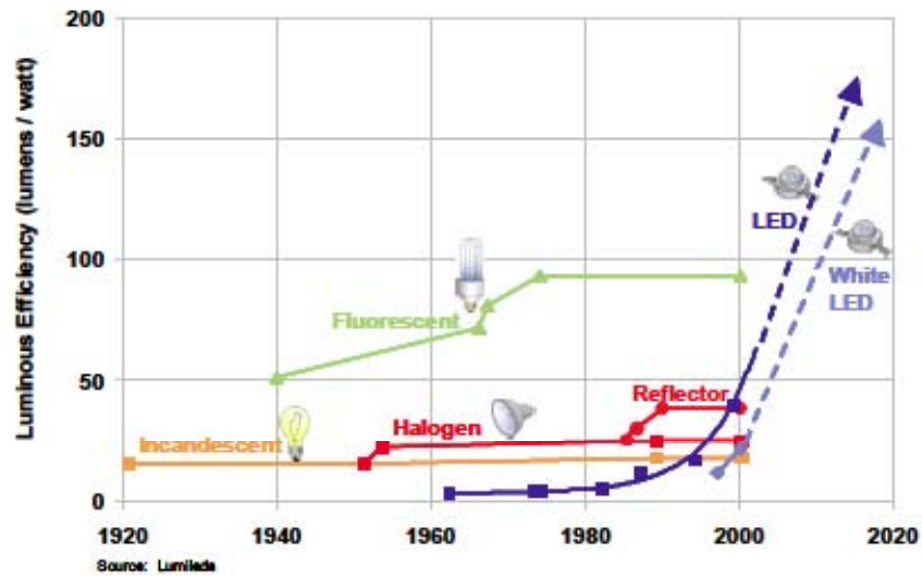
Figure 12. Increase in Lighting Efficiency from 1920 - 2020 (Navigant Consulting Inc., 2006)
