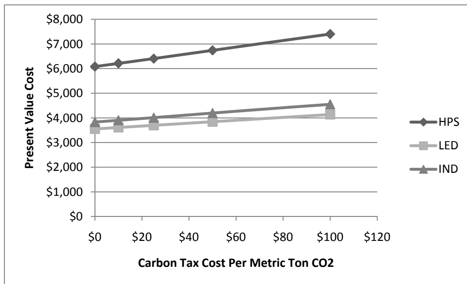
Figure 29. Carbon Emission Offset Cost Sensitivity with High Utility and Labor Rate (Clear AFS)
