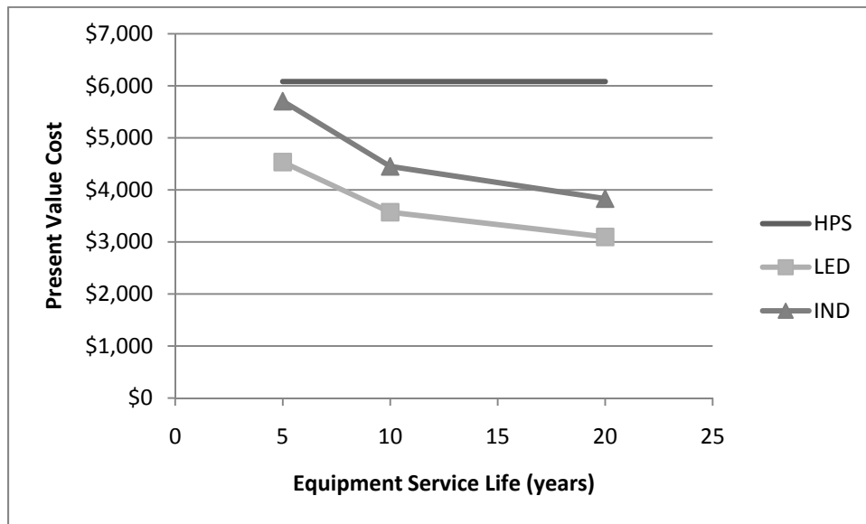
Figure 20. Equipment Service Life Sensitivity with High Utility and Labor Rate (Clear AFS)
