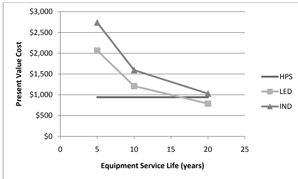
Figure 18. Equipment Service Life Sensitivity with Low Utility Rate (Hill AFB)
