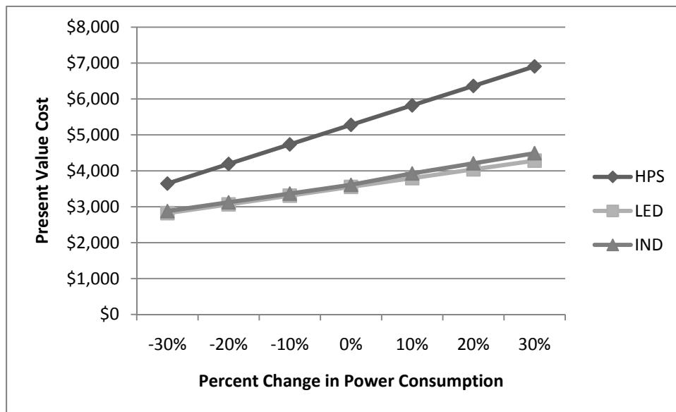
Figure 26. Power Consumption Sensitivity with High Utility and Labor Rate (Clear AFS)
