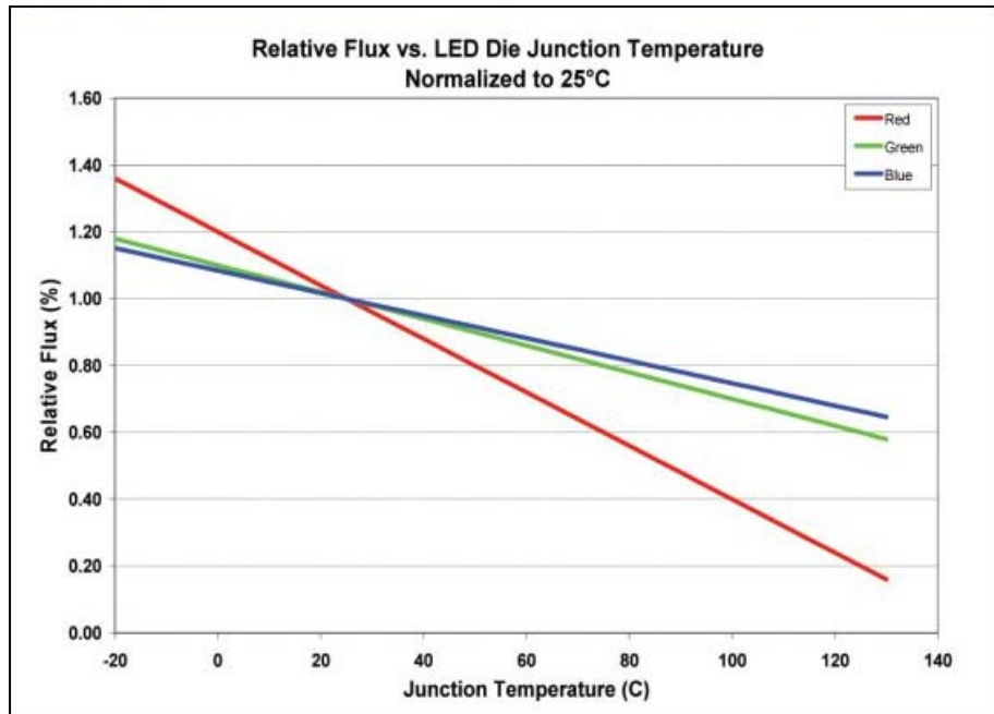
Figure 11. Relative Flux Vs LED Die Junction Temperature (Cooper, 2007)
