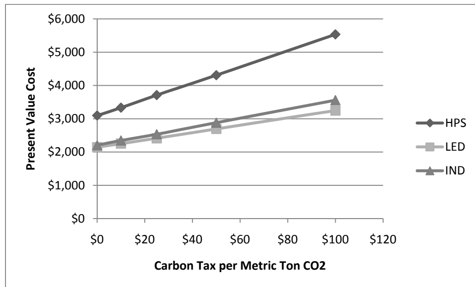
Figure 31. Carbon Emission Offset Cost Sensitivity for High CO 2 Emission Location (Bolling AFB)
