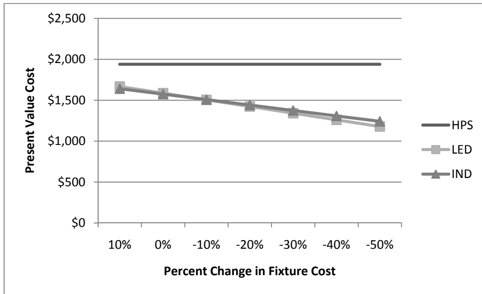
Figure 22. Fixture Cost Sensitivity with Low Labor Rate (Kirtland AFB)
