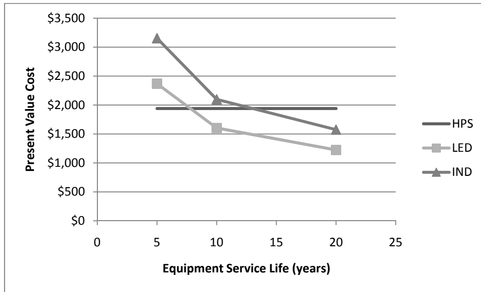
Figure 19. Equipment Service Life Sensitivity with Low Labor Rate (Kirtland AFB)
