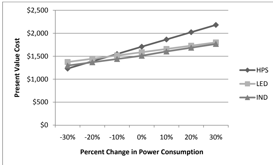
Figure 25. Power Consumption Sensitivity with Low Labor Rate (Kirtland AFB)
