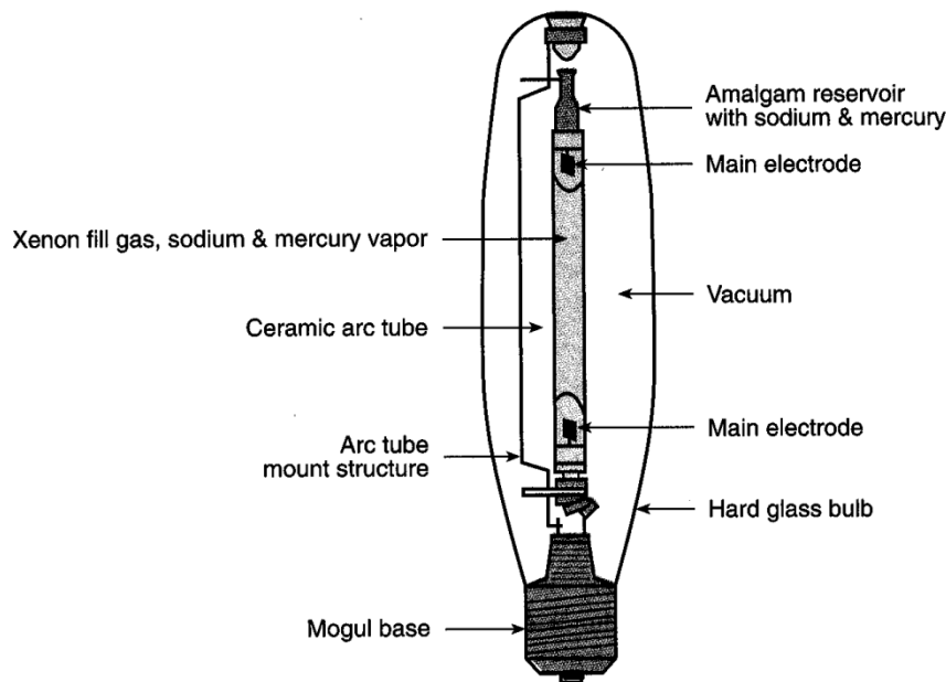
Figure 6. High-Pressure Sodium Bulb Components (Rea, 2000)
