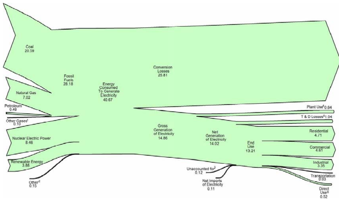
Figure 2. Electricity Flow, Quadrillion BTUs (EIA, 2008)
