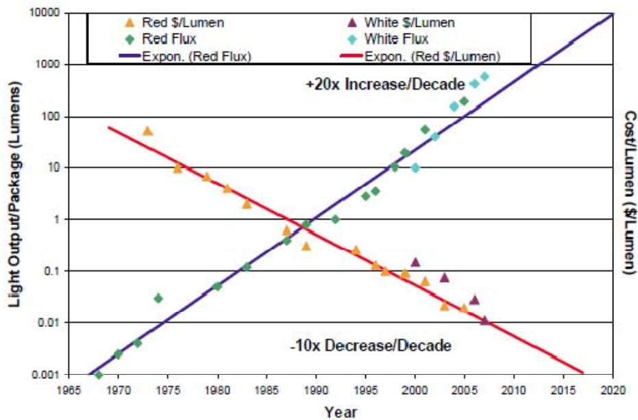
Figure 13. Light Output versus Cost (Navigant Consulting Inc., 2006)
