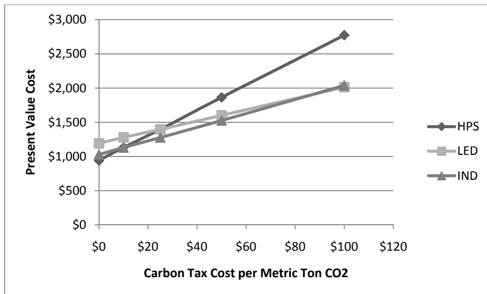
Figure 27. Carbon Emission Offset Cost Sensitivity with Low Utility Rate (Hill AFB)
