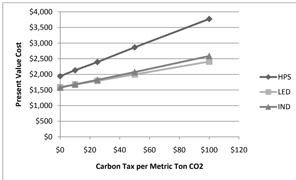
Figure 28. Carbon Emission Offset Cost Sensitivity with Low Labor Rate (Kirtland AFB)
