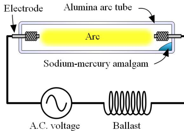
Figure 7. High Pressure Sodium Construction (Wikipedia, 2009)
