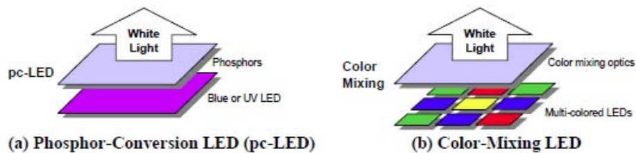
Figure 10. Methods for Making White LEDs
