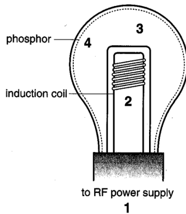
Figure 8. Induction Light (Rea, 2000)
