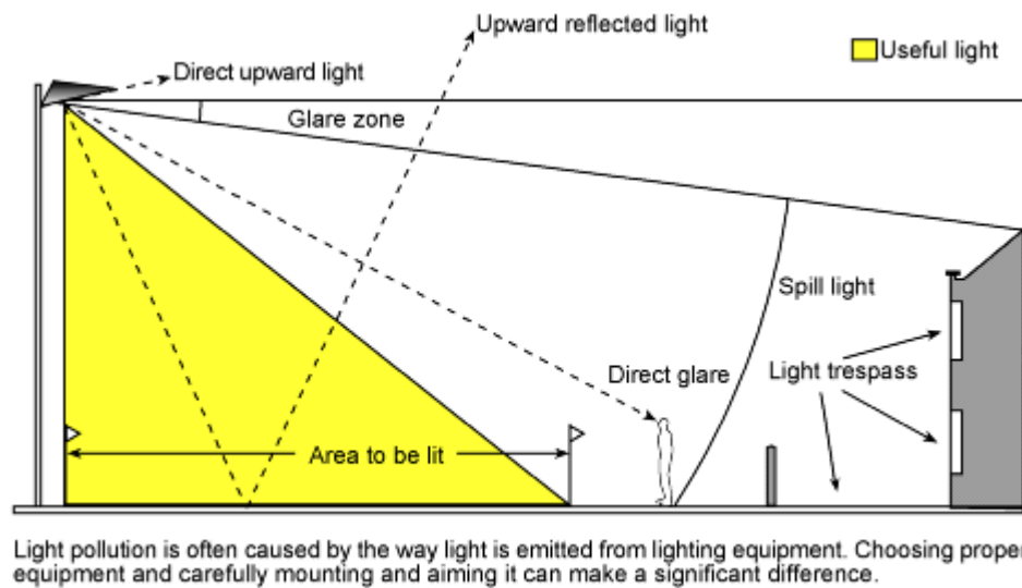
Figure 4. General Lighting Issues Associated with Street Lighting (Rensselaer Polytechnic Institute, 2007)
