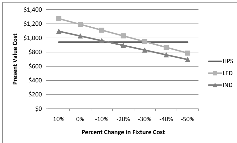
Figure 21. Fixture Cost Sensitivity with Low Utility Rate (Hill AFB)
