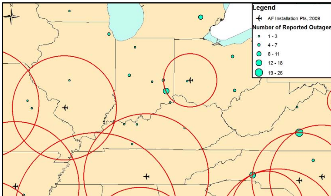
Figure 10. IDW for a Sample set of Air Force Installations
