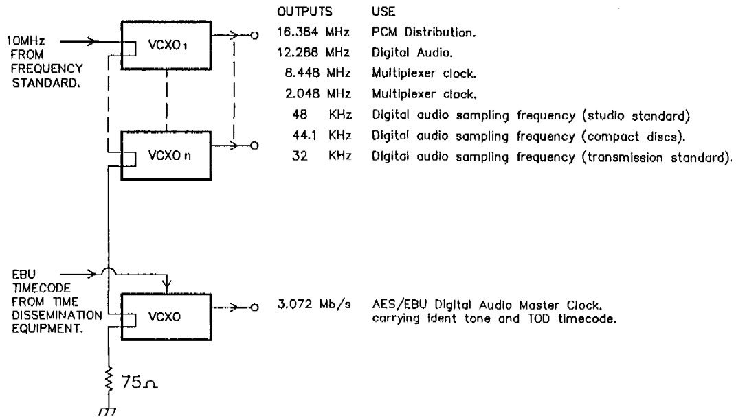
Figure 3 : Frequency Dissemination.
