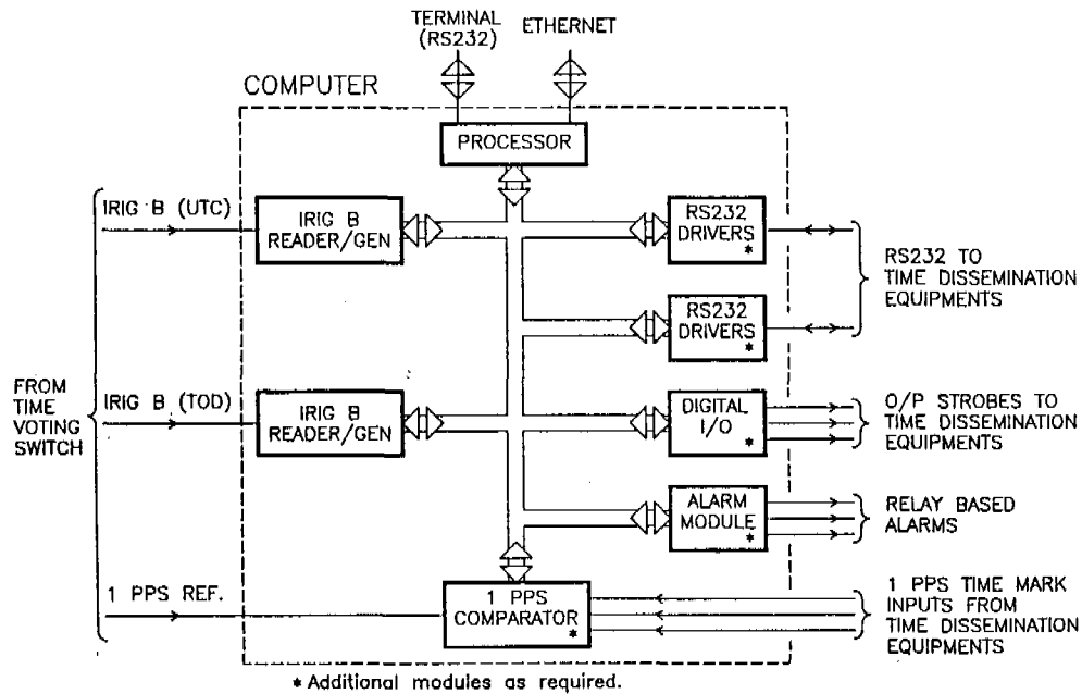
Figure 4: System Computer
