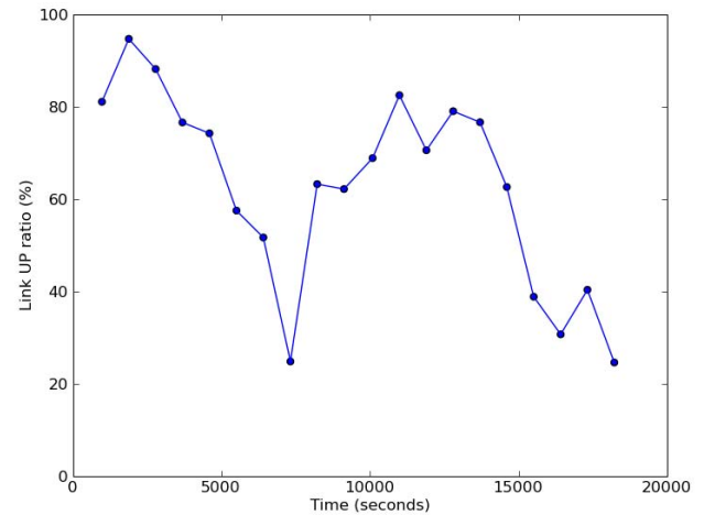
Figure 10: Percentage of time OSPF link between nodes 166 and 167 was in two way or fully connected.
