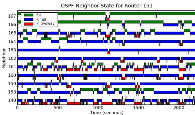
Figure 9: Link status for the ground mobile node
