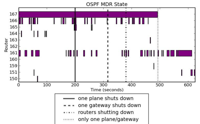
Figure 7: MDR status of the network nodes.
