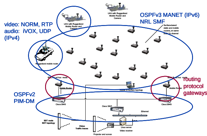
Figure 1: Demonstration topology
