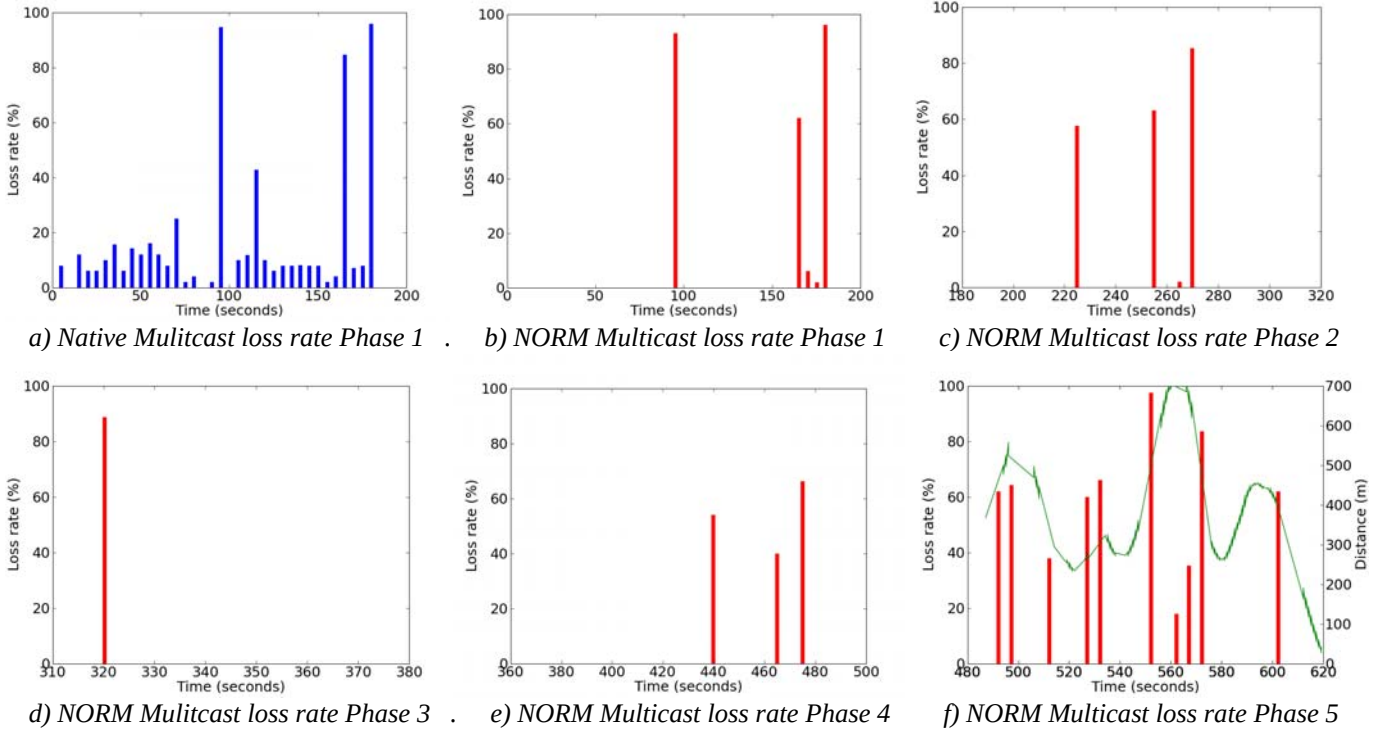
Figure 6: Multicast loss rate during the flight test.
