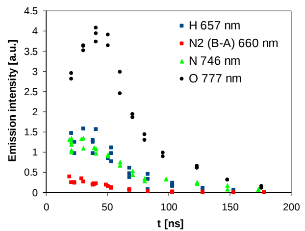
Figure 37. Temporal evolution of the emission intensity of the TS measured by ICCD at specific wavelengths.
