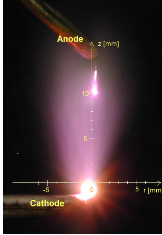
Figure 19. DC glow discharge in air preheated to \sim 2000 K: I=100 mA, gap 1 cm, vertical upward flow, v=278 m/s.
