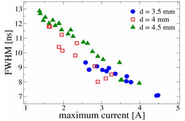
Figure 30. Full width of the pulse at half maximum (FWHM) as a function of the maximum current in the pulse ( I_{max} ).
