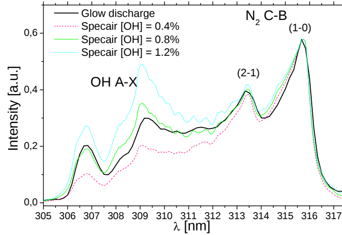
Figure 18. Fitting OH bands to estimate the OH concentration in the glow discharge. Gap: 4 mm; I=6 mA.
