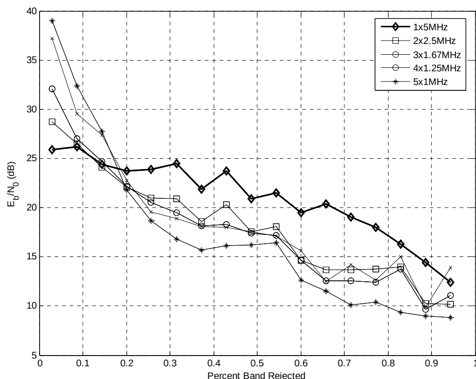
Figure 4 Required E_b/N_0 to achieve an error rate of 10^{-3} as a function of the percent band rejected.
