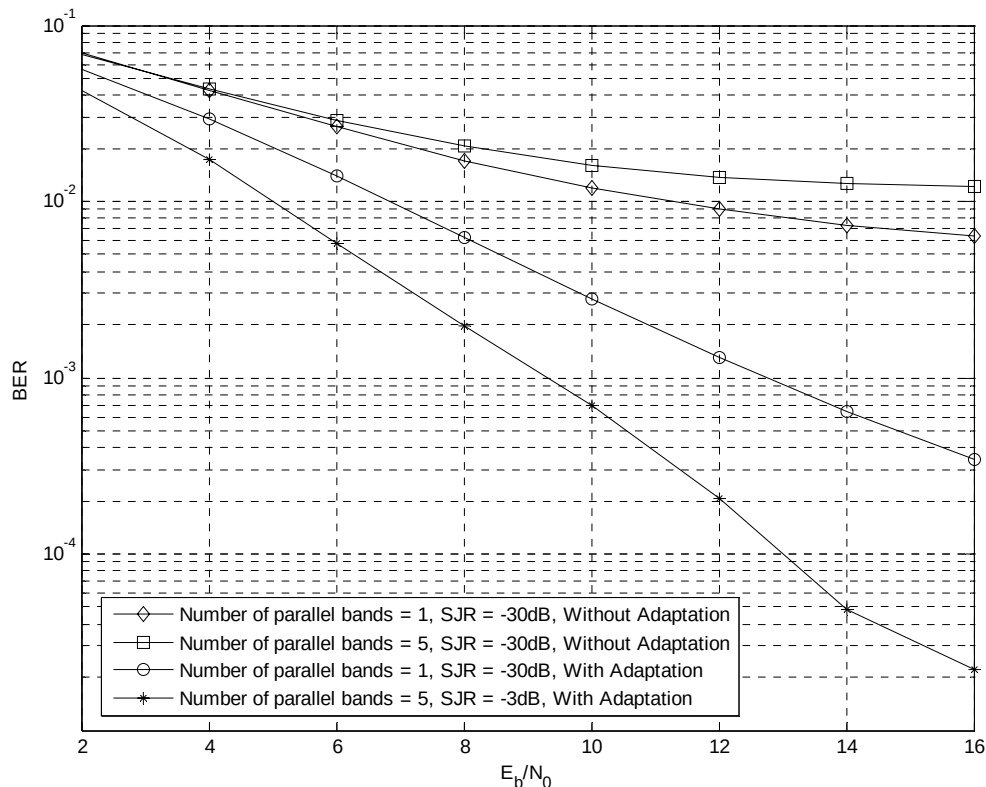
Figure 5 BER performance of the multi-band transmission scheme with and without spectrum adaptation.
