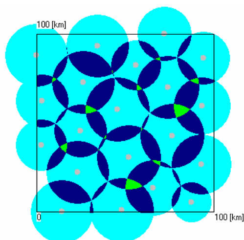
Figure 8. The final result of global power optimisation
