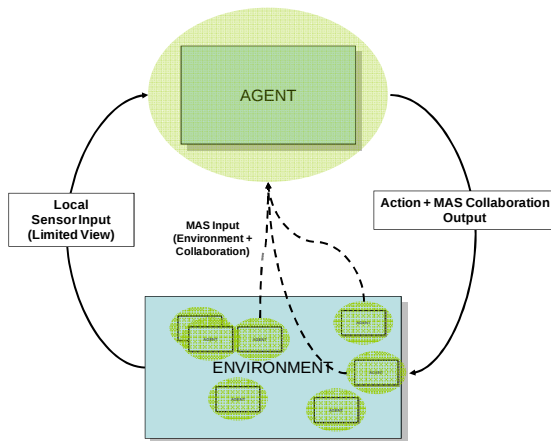
Figure 2: MAS Interactions
