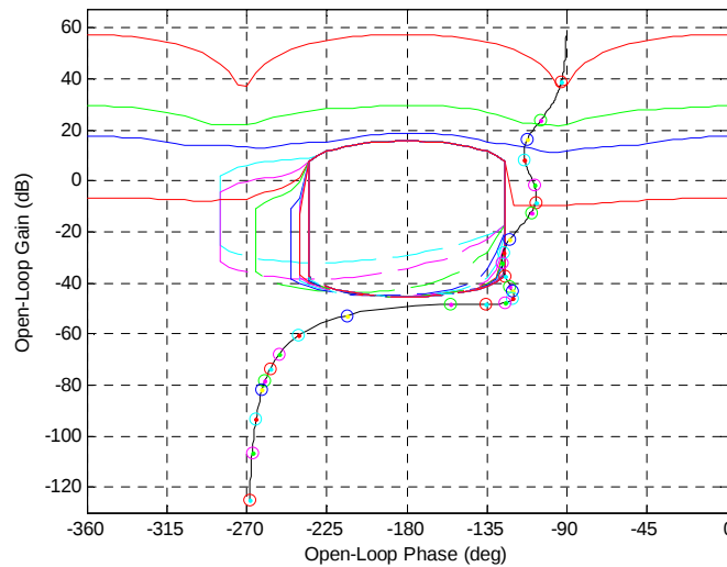
Fig.7. Nichols plot for L_o(s) with G_1(s)
