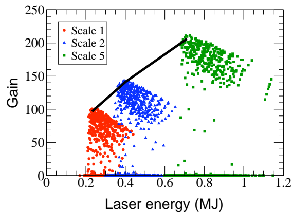
Figure 1: Results of one-dimensional simulations showing the fusion energy gain as a function of KrF laser energy for three classes of shock-ignited target designs. As explained in the text, the scale-1 target (red circles) serves as the baseline design in this study; the other two classes of pellets have total masses that are two and five times larger.
