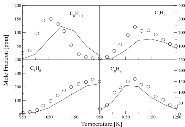
Figure 4.5 Concentration profiles of intermediate species during n-propyl benzene oxidation in a jet-stirred reactor with \Phi = 1.0 , P = 1 atm, T = 950 - 1250 K. The circles are measurements [96] and the solid line the current simulation.
