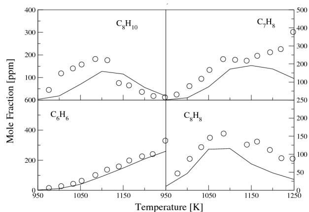
Figure 4.8 Concentration profiles of intermediate species during n-propyl benzene oxidation in a jet-stirred reactor with \Phi = 1.5 , P = 1 atm, T = 950 - 1250 K. The circles are measurements [96] and the solid line the current simulation.
