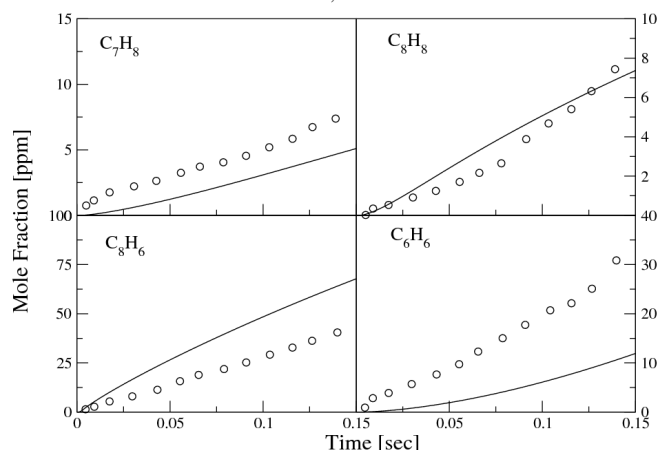
Figure 5.18 Concentration profiles of major species during 1-methyl naphthalene oxidation in a flow reactor ( \Phi = 1.0 , P = 1 atm, T = 1169 K). Circles indicate measurements [119] and solid lines the current computations
