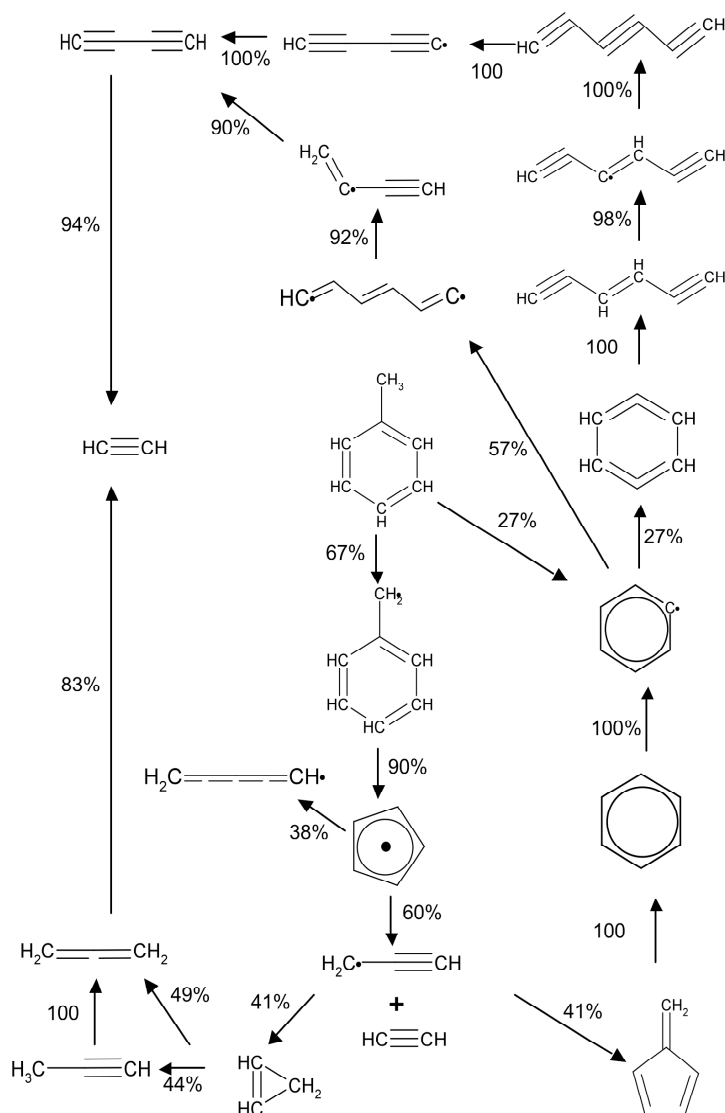
Figure 3.12 Predicted toluene thermal decomposition pathways corresponding to the study of Braun-Unkhoff et al. [77] with an initial fuel concentration of 2.0 ppm, T = 1515 K and P = 1.85 bar.
