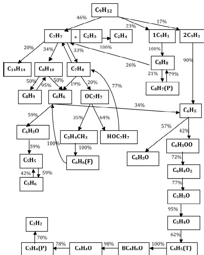
Figure 4.11. n -Propyl benzene oxidation pathways for \Phi = 1.5 , T = 1050 K and P = 1 atm in a jet stirred reactor
