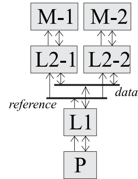
Figure 2. One possibility of the new cache/memory structure
