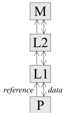
Figure 1. Typical 2-level cache design
