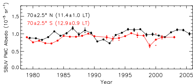
Figure 9. SBUV PMC albedos at 252.0 nm from opposite hemispheres analyzed herein. The 70°N albedos are reproduced from Figure 5 for comparison.
