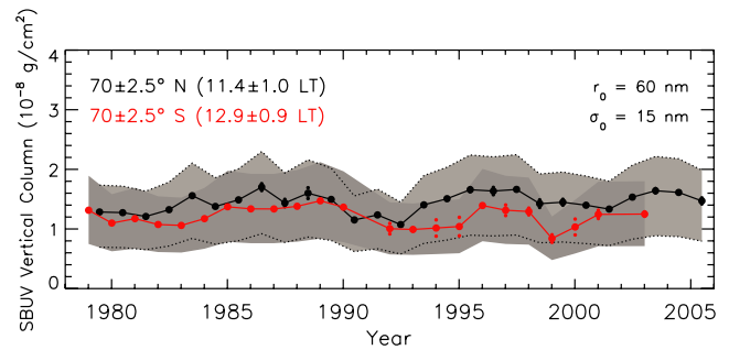
Figure 10. Vertical water ice column inferred from SBUV PMC data in opposite hemispheres. Characteristics of the particle size distribution are indicated in the upper right and are the same for both hemispheres.
