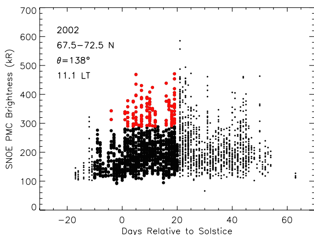
Figure 3. Example of one northern season (2002) of SNOE PMC data between 67.5 and 72.5^\circ\text{N} . Each symbol represents a PMC observation. Large circles are the data over the time period used in this study. Large red circles are the brightest SNOE PMCs that on average match the SBUV cloud frequency and are therefore representative of the SBUV observations. These brightest PMCs are 10% of all SNOE PMC observations between -10 and 20 DRS.
