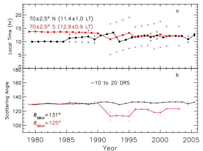
Figure 2. (a) SBUV LT comparison between Northern Hemisphere data (black, Figure 1) and Southern Hemisphere data (red) used in this work. (b) Solar scattering angle comparison for the Northern (black) and Southern Hemisphere data (red). The average scattering angles are indicated.
