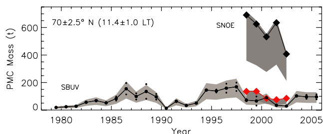
Figure 7. Annually averaged PMC ice mass. The shaded areas represent the uncertainty in the characteristics of the size distribution indicated in Figure 6. All solutions shown use the same size distribution as indicated in the upper right of Figure 6.
